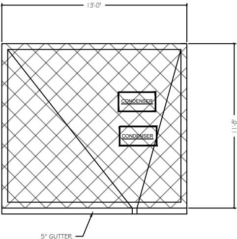
BULKHEAD ROOF FLOOR PLAN
