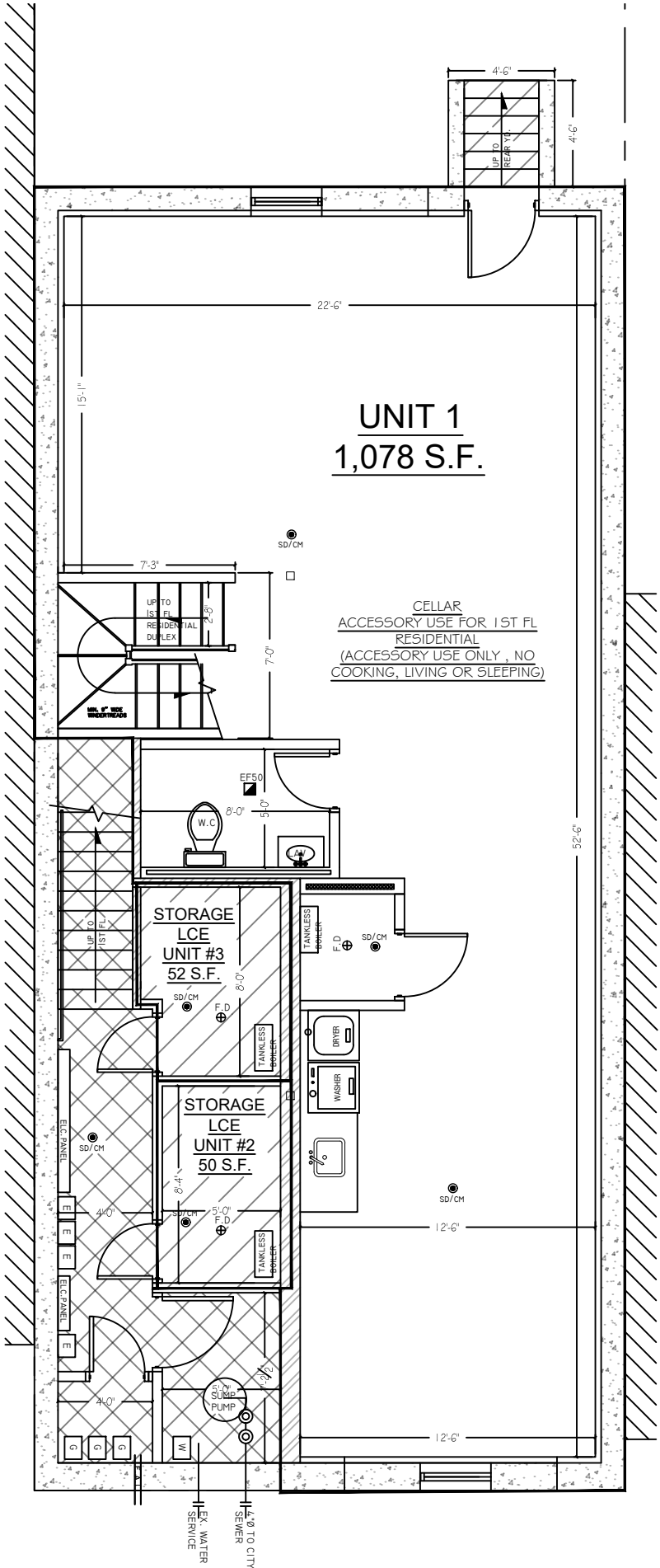
CELLAR FLOOR PLAN
