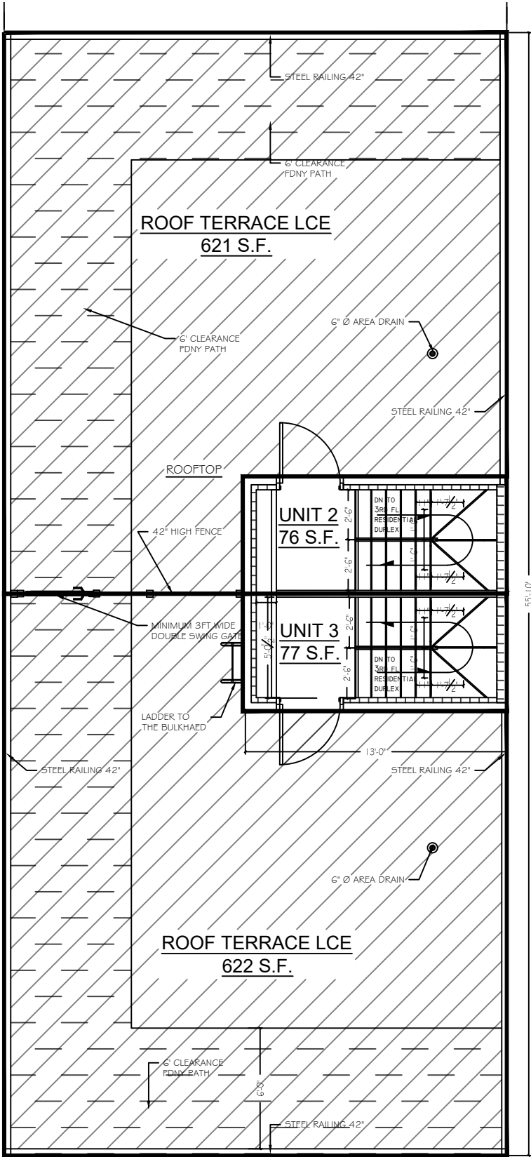
ROOF FLOOR PLAN
