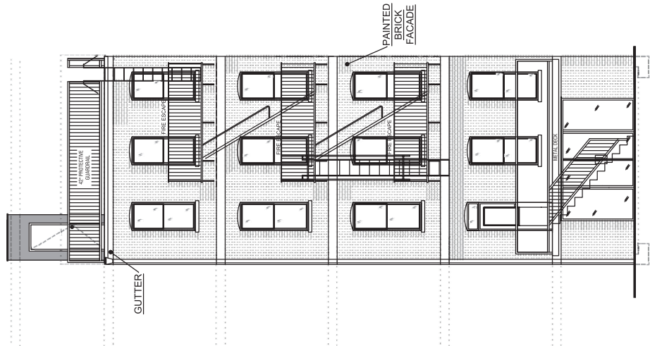
REAR ELEVATION
