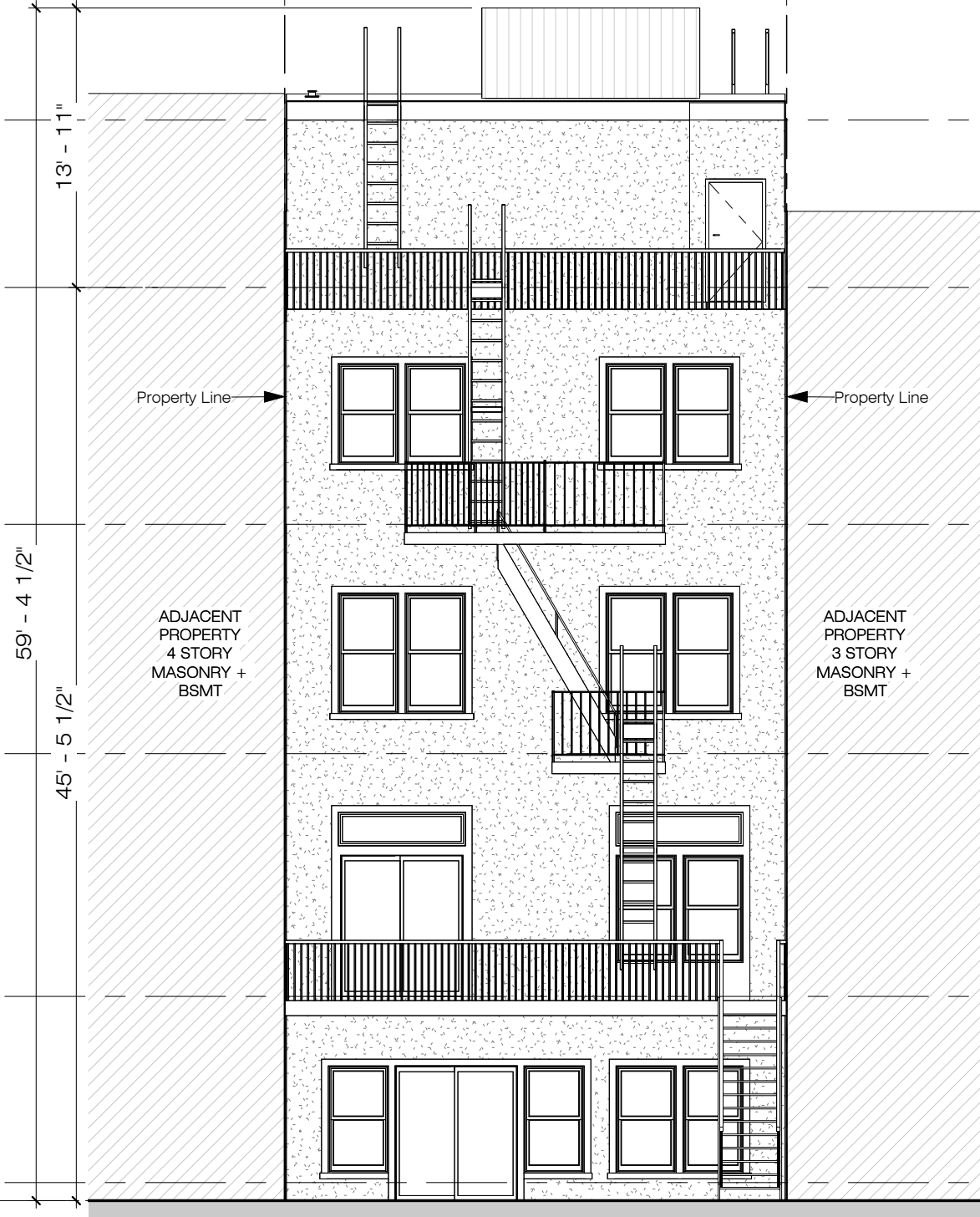
② PROPOSED REAR ELEV 1/8" = 1'-0"
