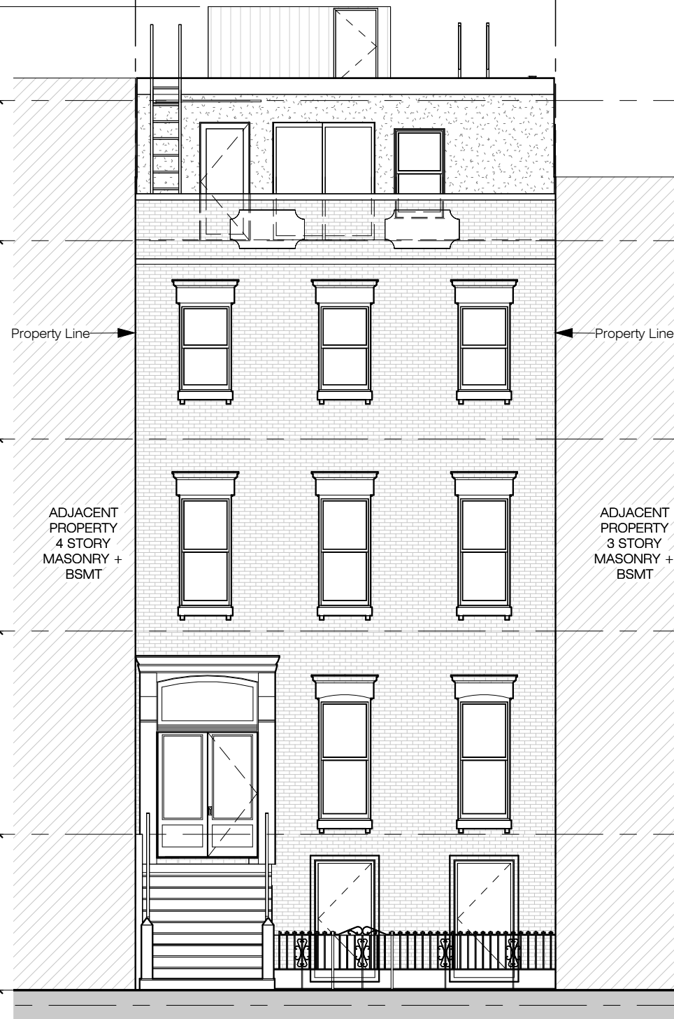
① PROPOSED FRONT ELEV 1/8" = 1'-0"
