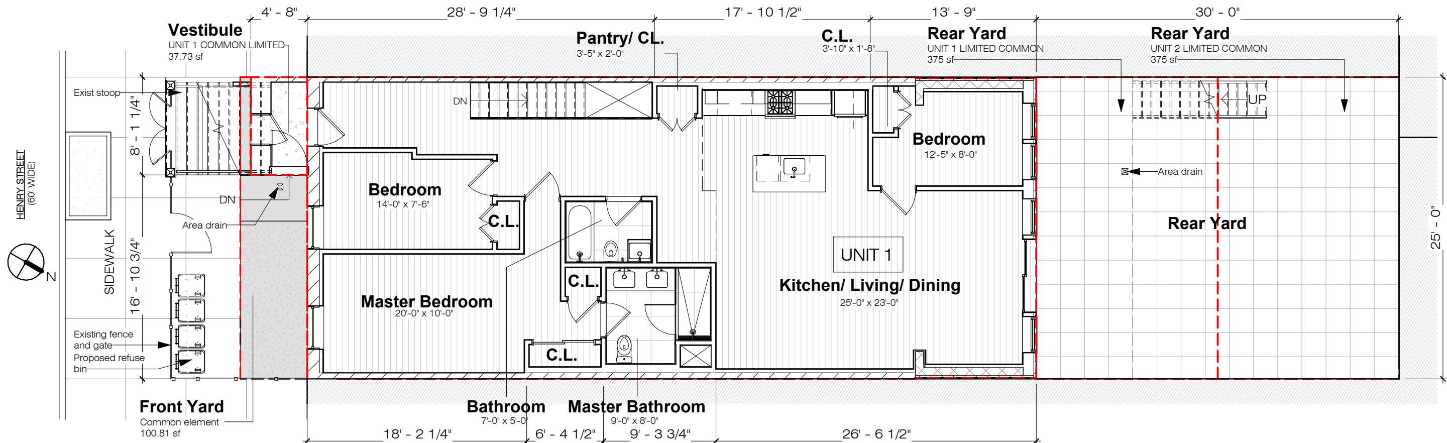
1 BASEMENT FL. OFFERING PLAN 1/8" = 1'-0"
