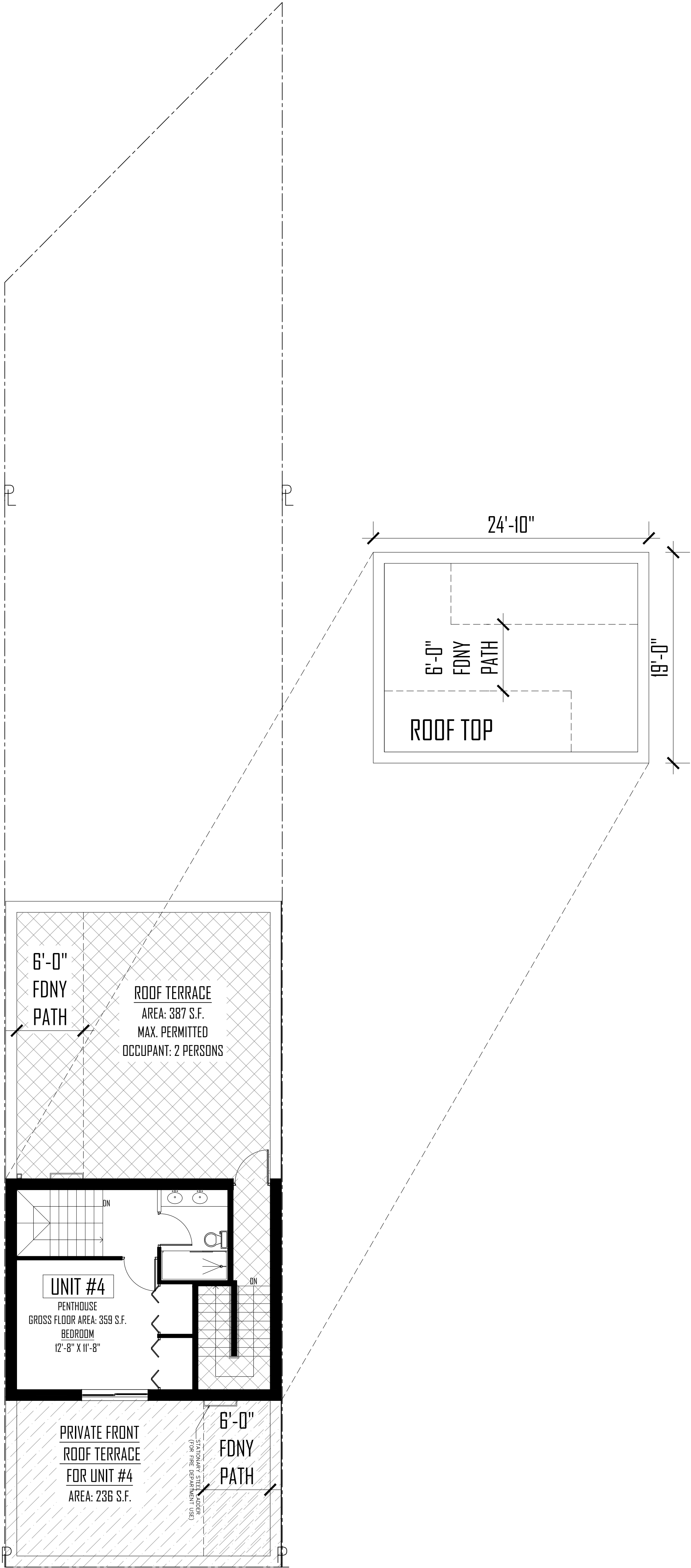
GARFIELD PLACE PENTHOUSE PLAN SCALE: 1/16" = 1'-0"
