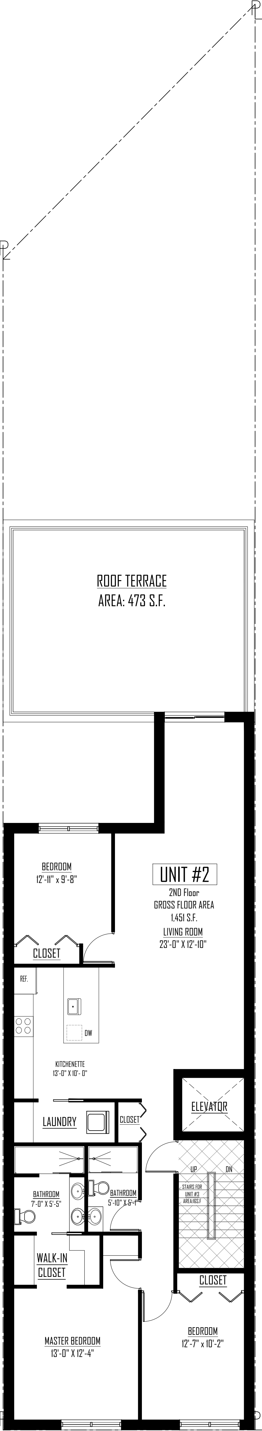
GARFIELD PLACE 2ND FLOOR PLAN SCALE: 1/16" = 1'-0"
