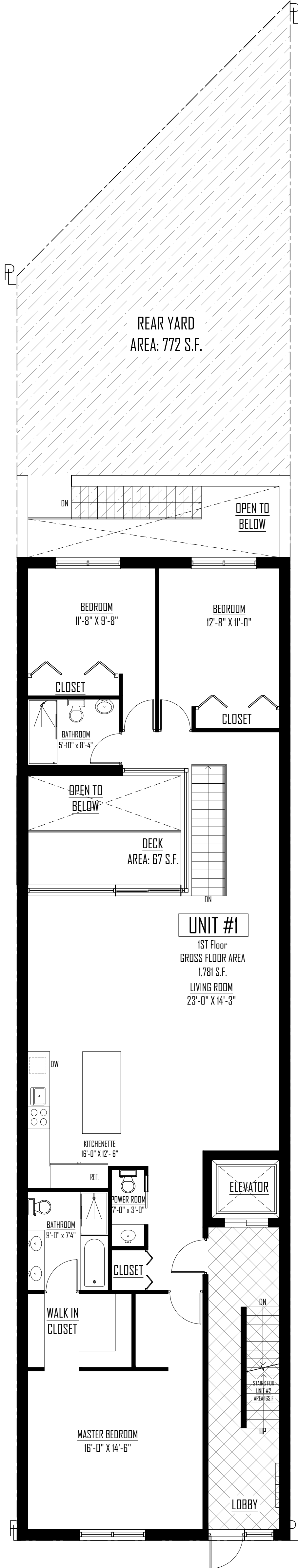
GARFIELD PLACE 1ST FLOOR PLAN SCALE: 1/16" = 1'-0"
