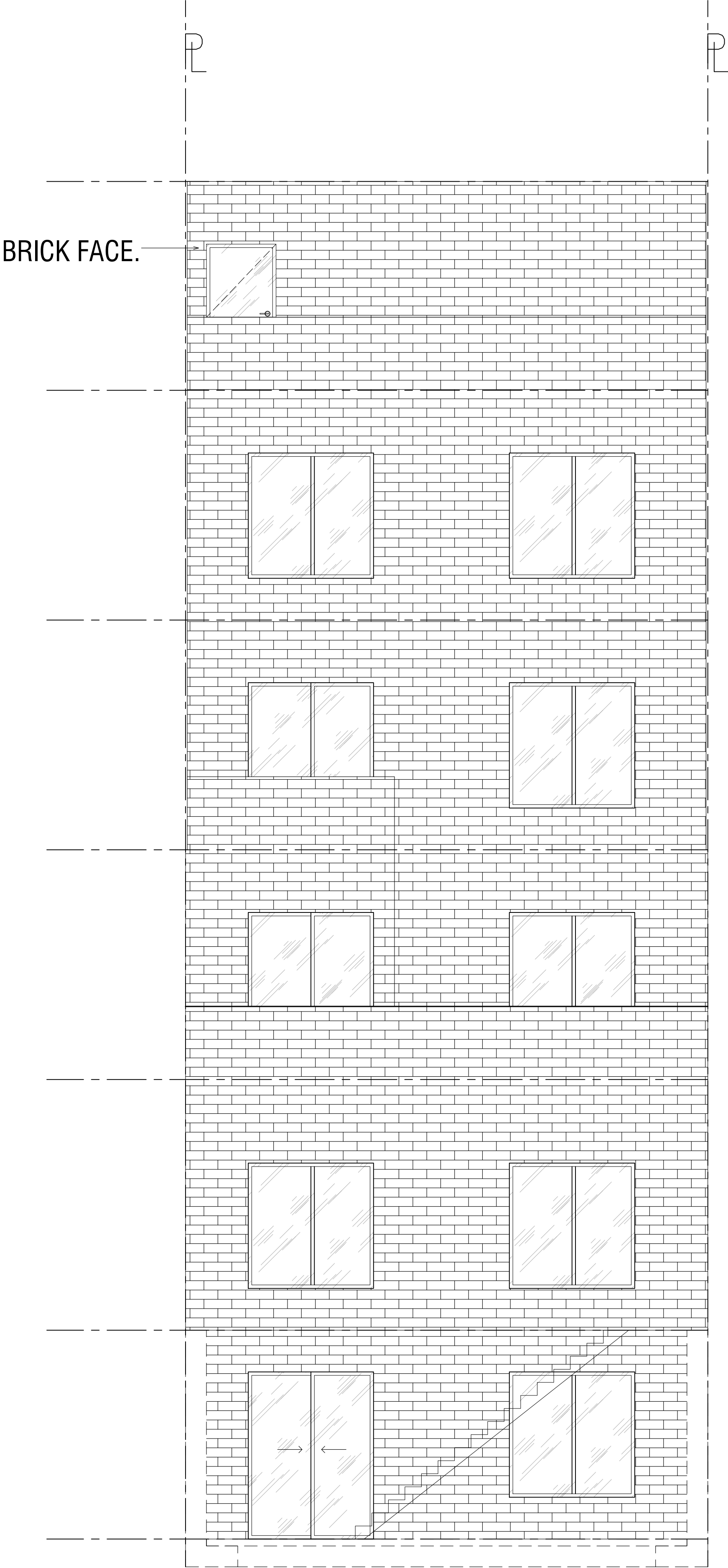
GARFIELD PLACE REAR ELEVATION PLAN SCALE: 3/32" = 1'-0"
