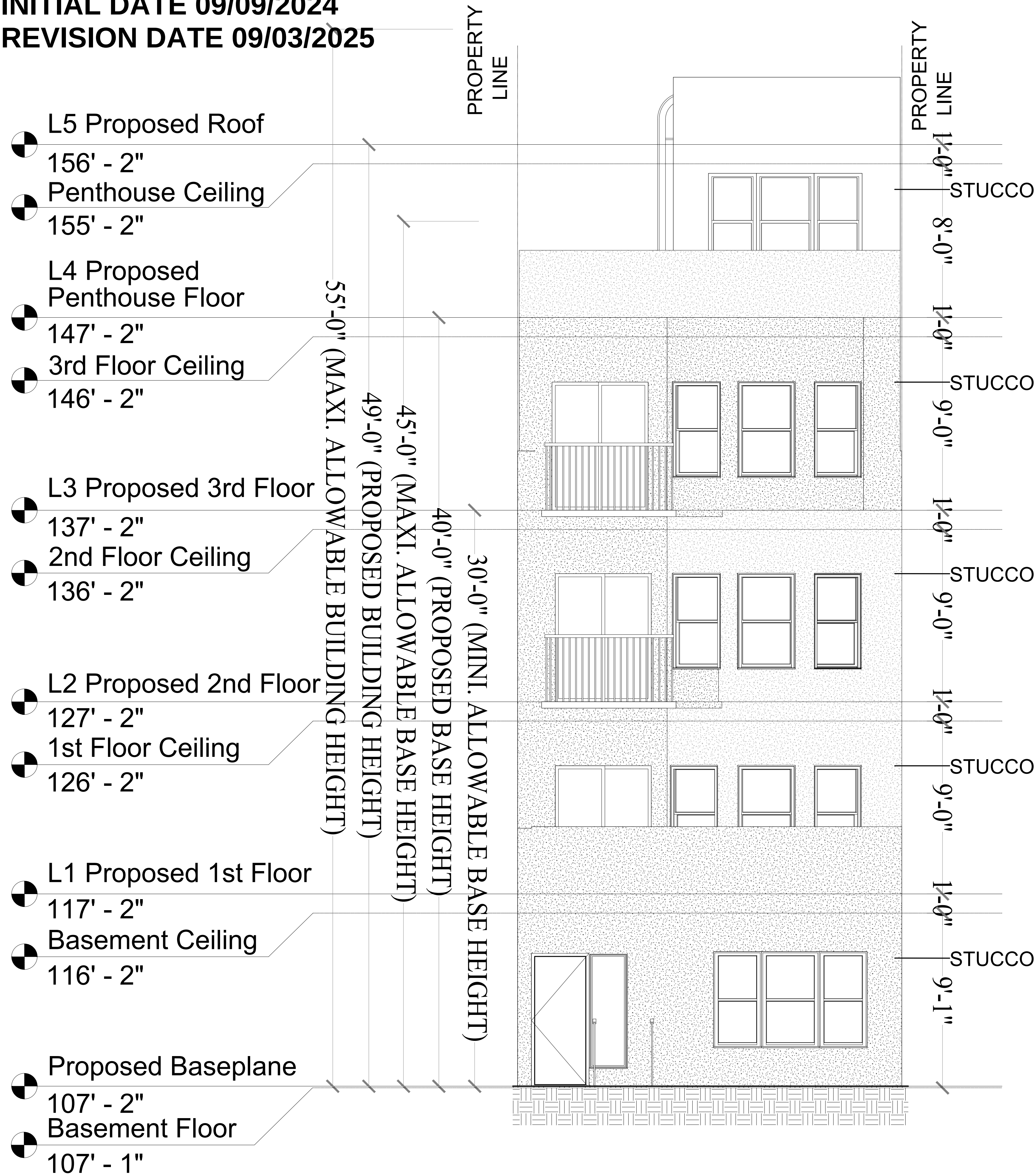
FRONT ELEVATION (NORTH)
