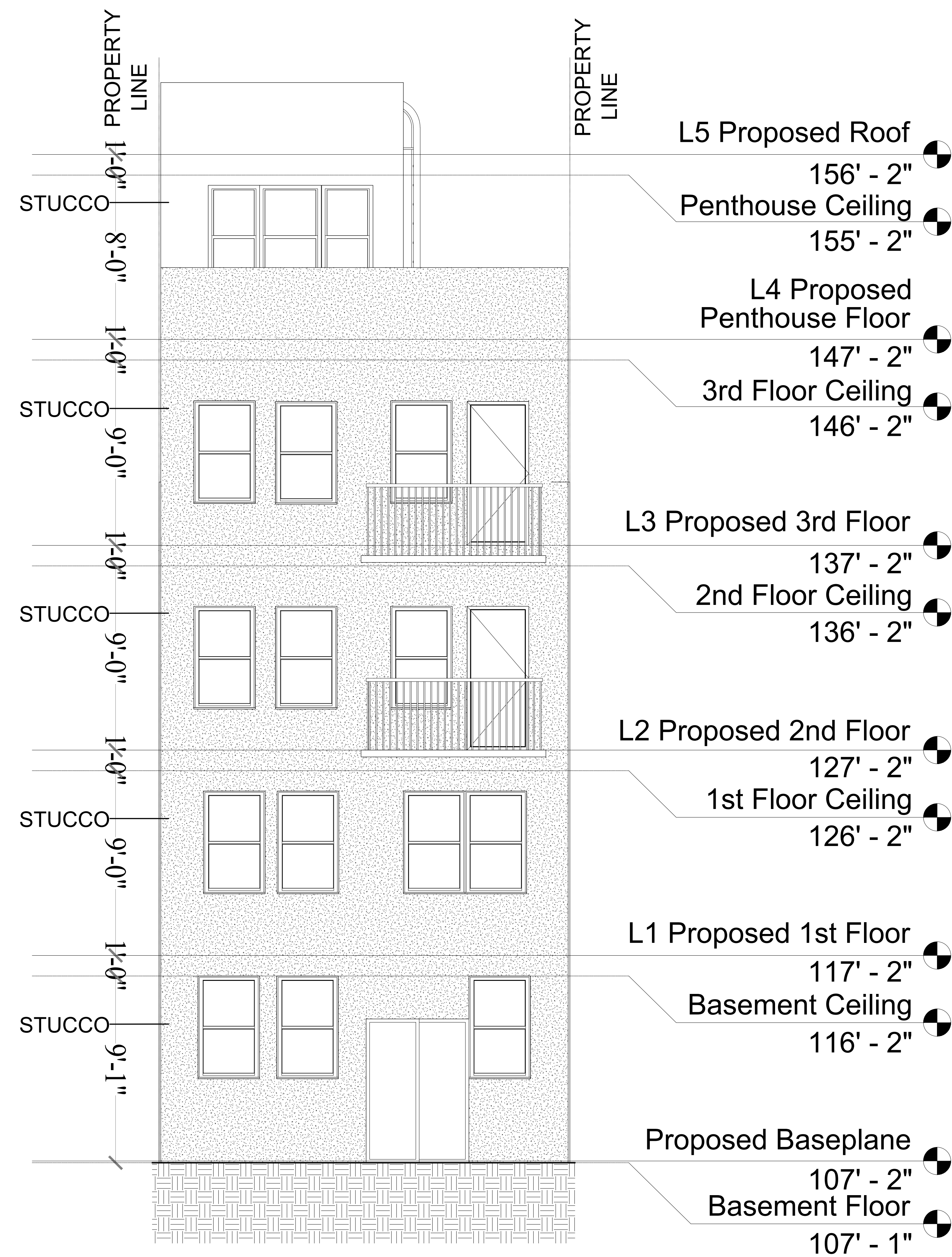
BACK ELEVATION (SOUTH)
