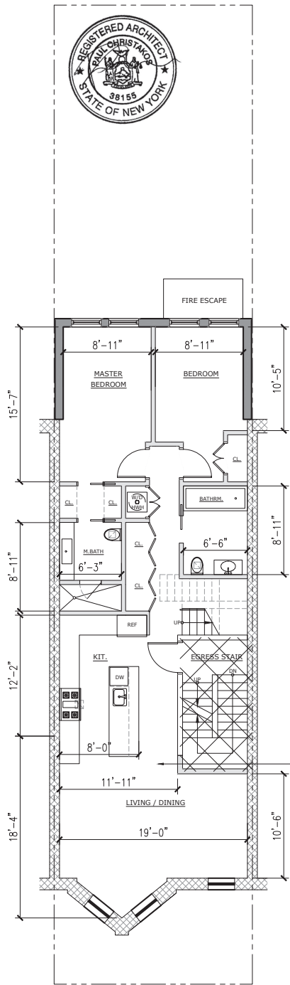
1 THIRD FLOOR PLAN SCALE: 1/8"=1'-0"
