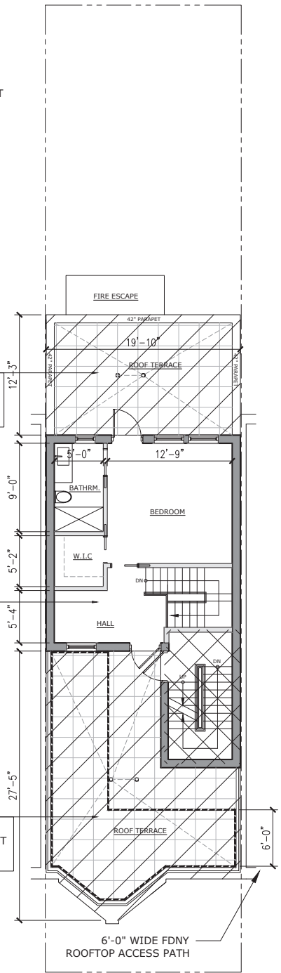
2 FOURTH FLOOR PLAN SCALE: 1/8"=1'-0"
