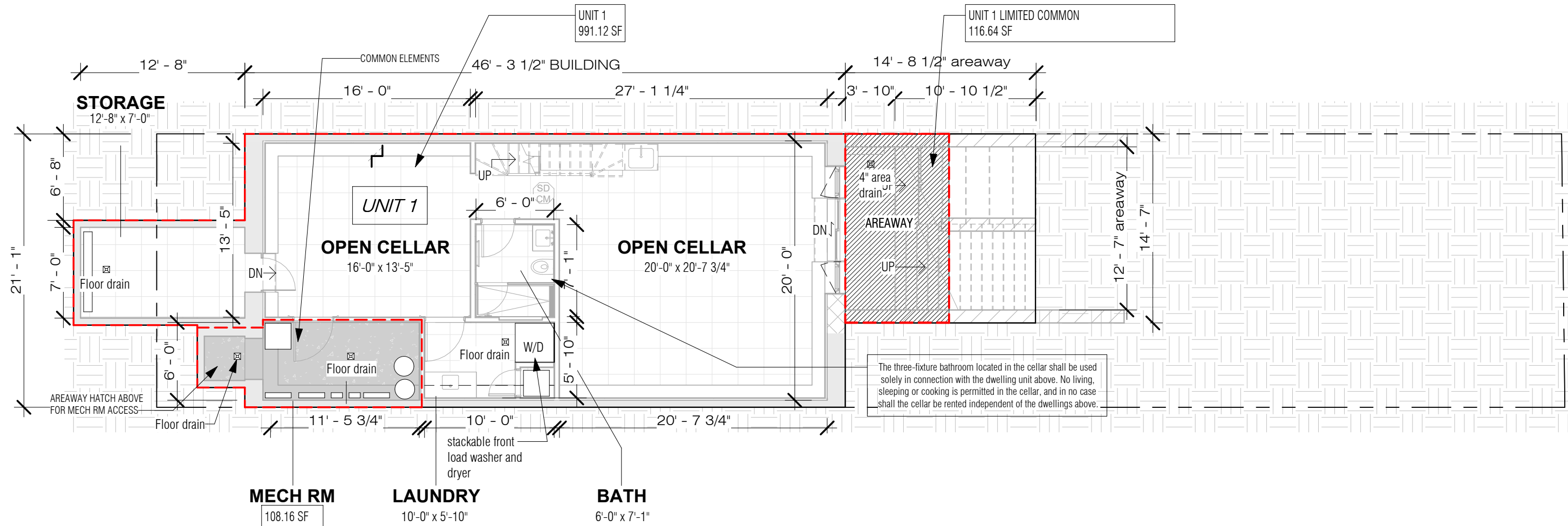
② OFFERING CELLAR PLAN 1/8" = 1'-0"
