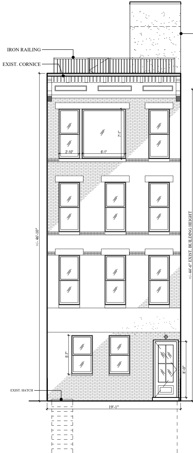
FRONT ELEVATION
