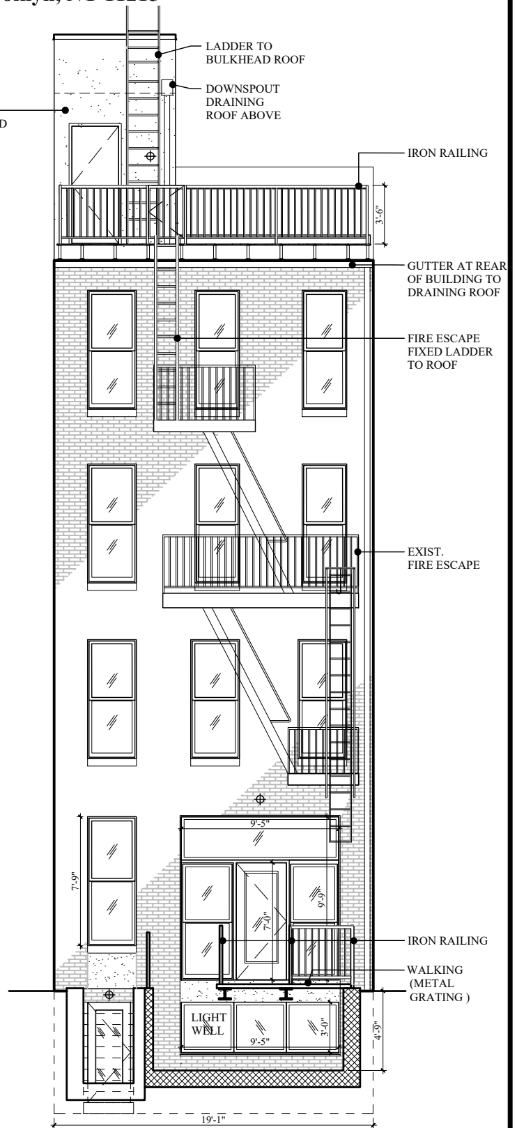
REAR ELEVATION
