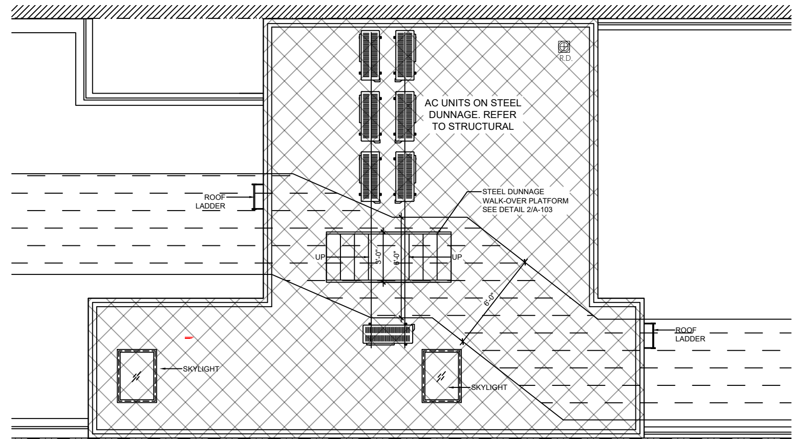
BULKHEAD FLOOR PLAN
