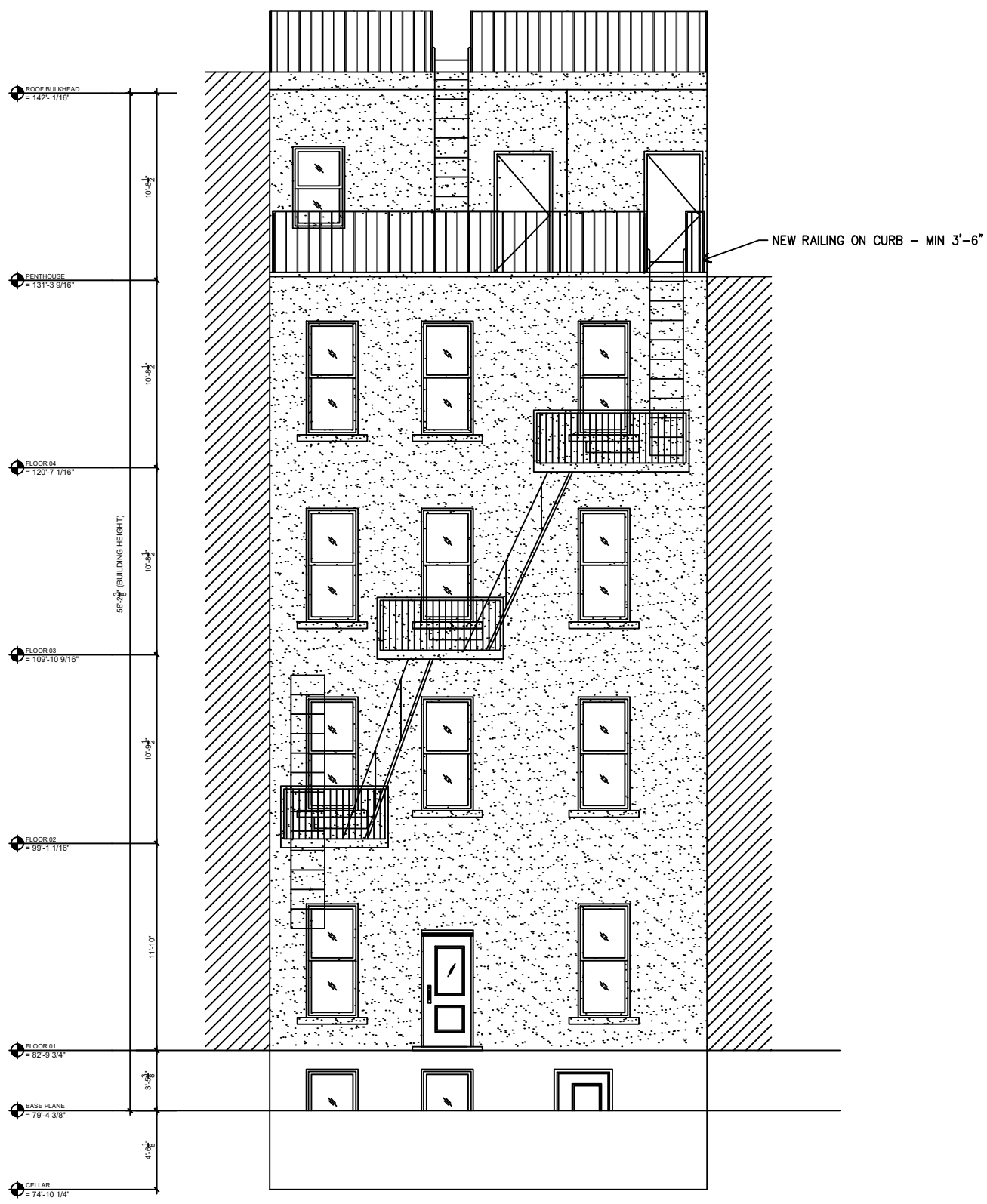
2 REAR SIDE ELEVATION A-201
