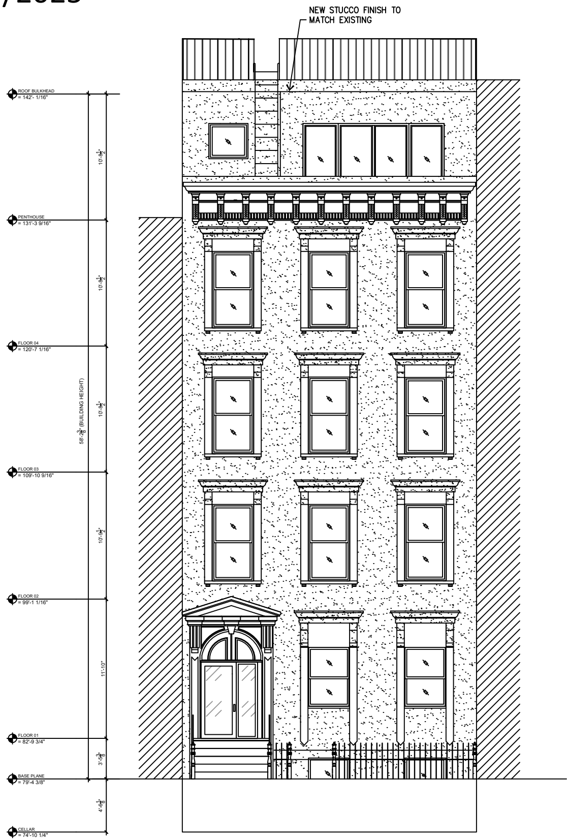
1 FRONT SIDE ELEVATION A-201
