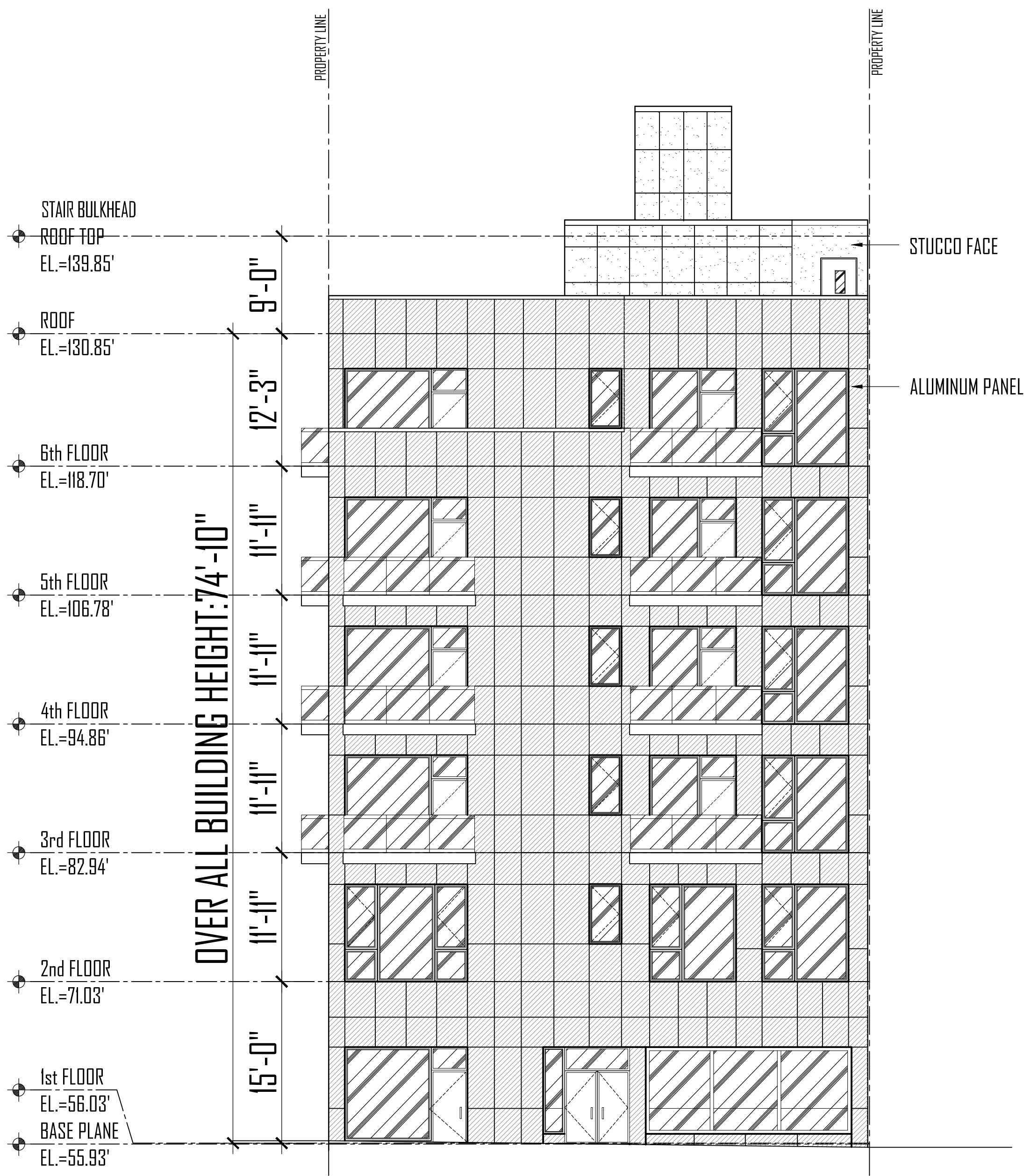
BUSHWICK AVENUE FRONT ELEVATION SCALE: 1/16"=1'-0"
