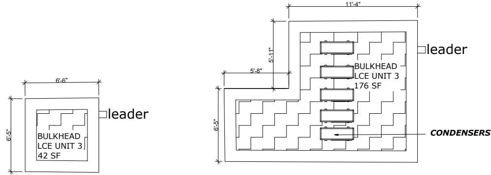
BULKHEAD FLOOR PLAN BULKHEADS SHALL NOT BE ENCLOSED BY PARAPETS OR RAILINGS.
