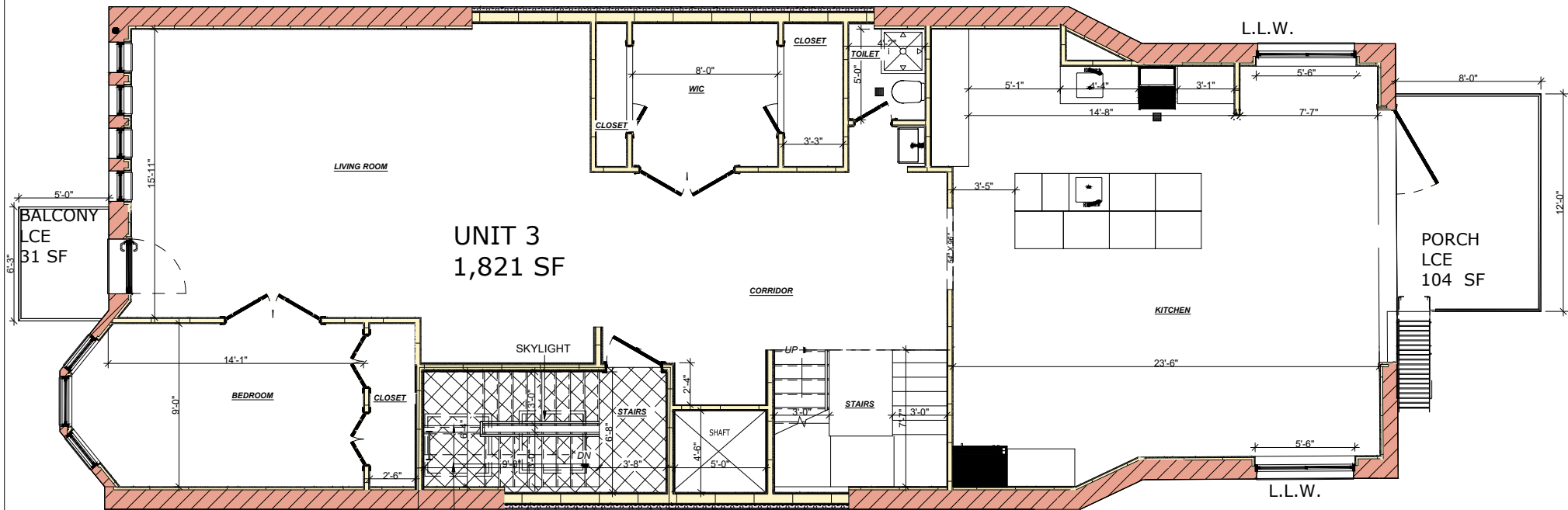
4TH FLOOR PLAN-UNIT 3
