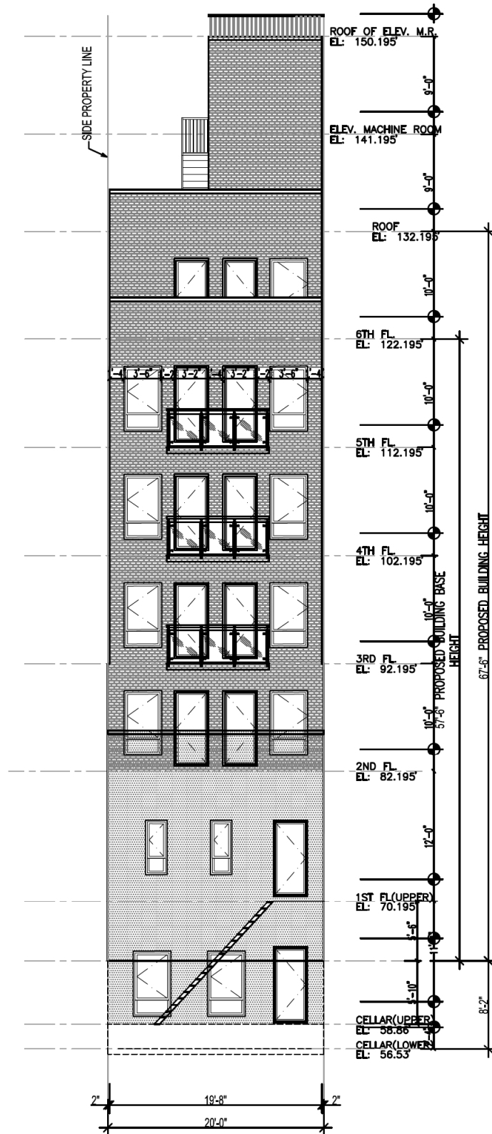
REAR ELEVATION
