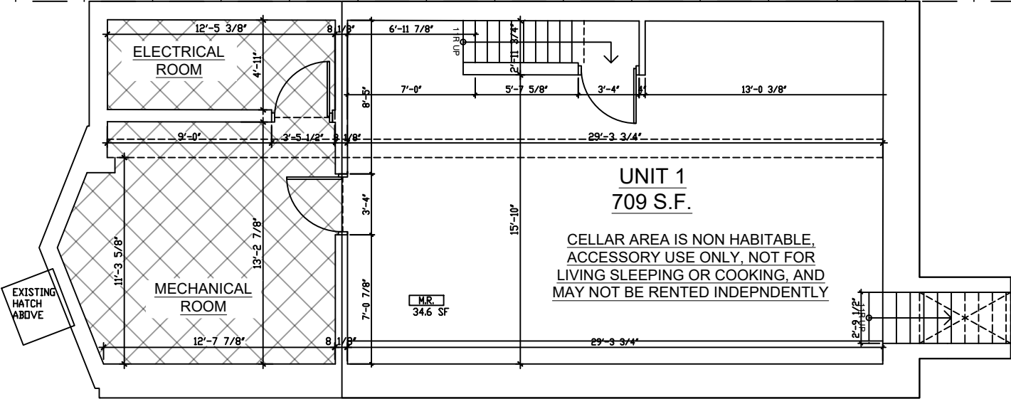
CELLAR FLOOR PLAN
