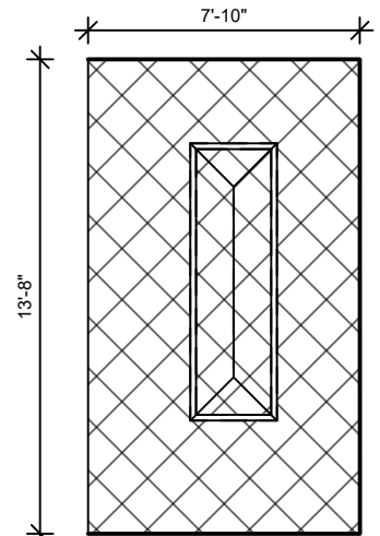
BULKHEAD FLOOR PLAN
