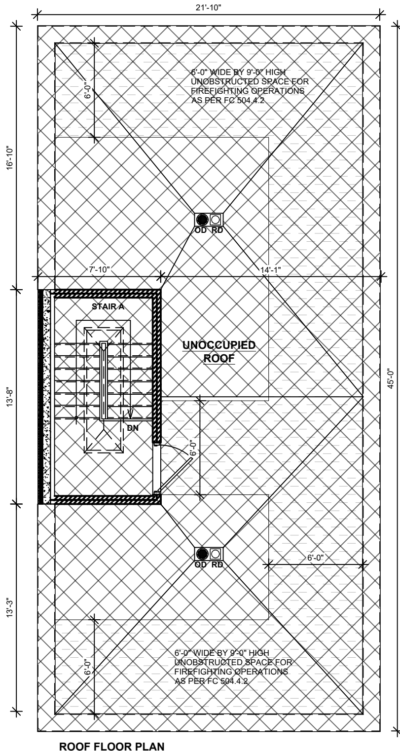
ROOF FLOOR PLAN
