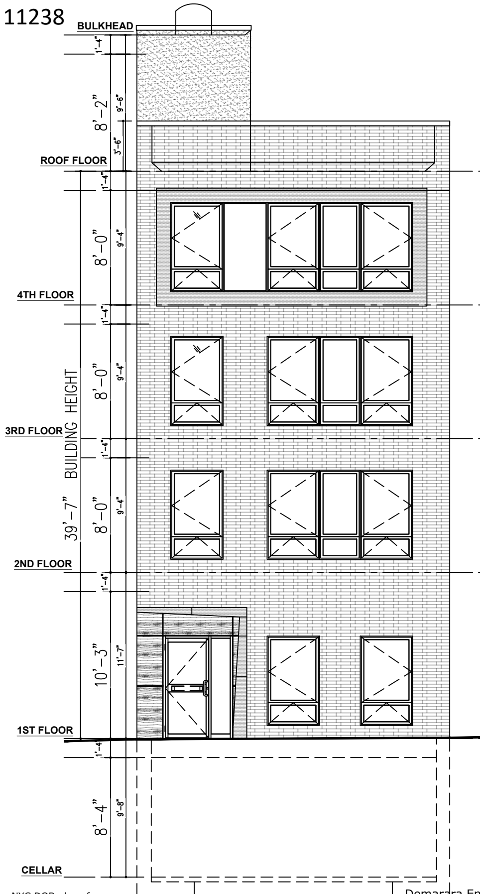
FRONT ELEVATION
