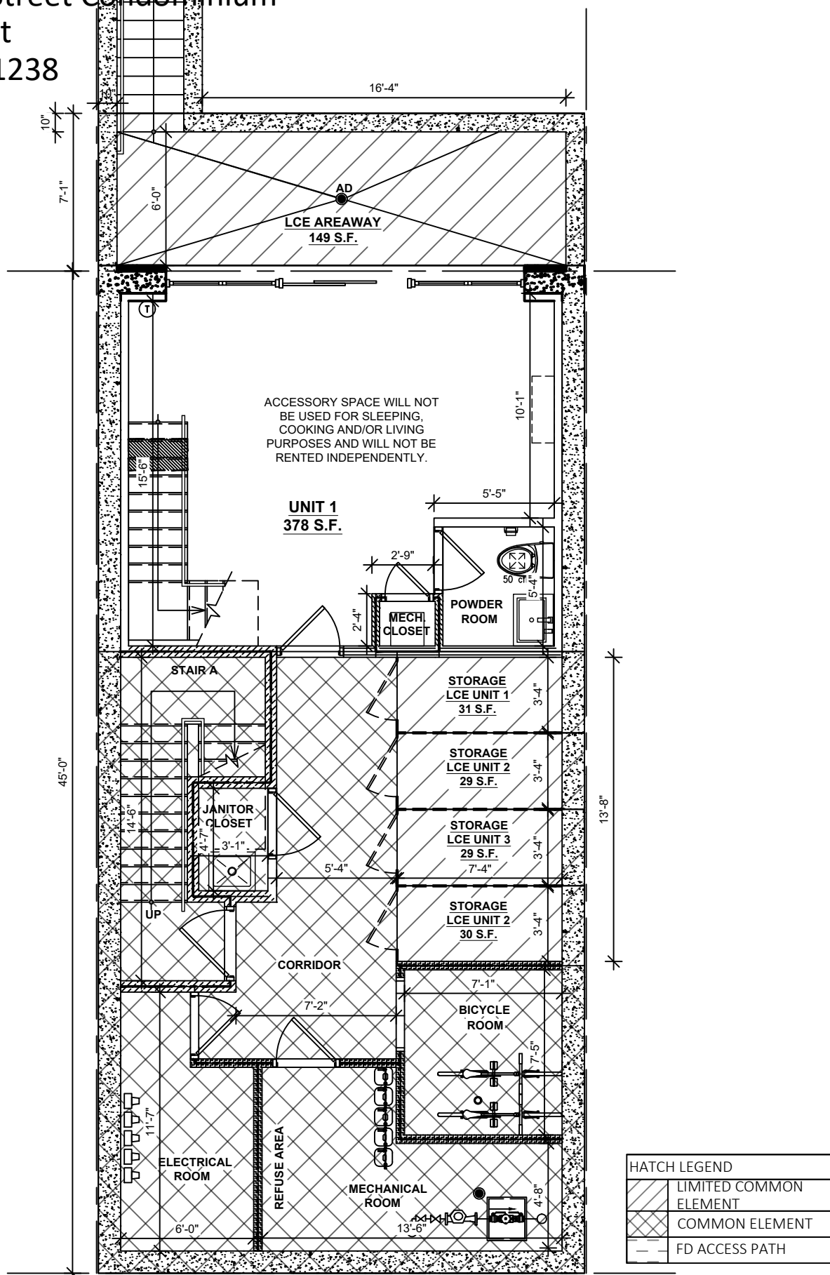
CELLAR FLOOR PLAN
