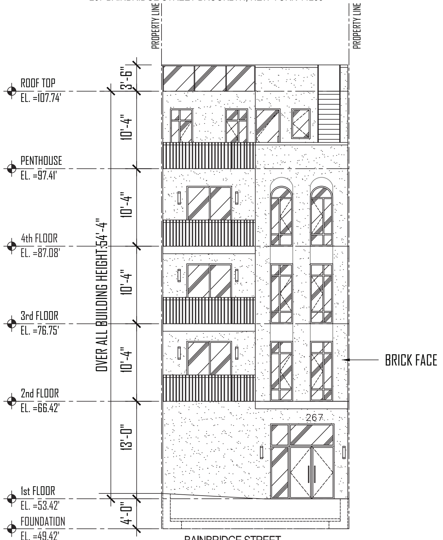
BAINBRIDGE STREET FRONT ELEVATION PLAN SCALE: 1/8" = 1'-0"
