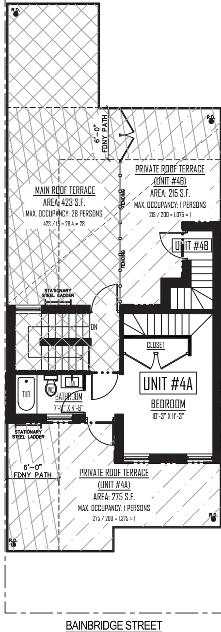
PENTHOUSE FLOOR PLAN SCALE: 3/32" = 1'-0"
