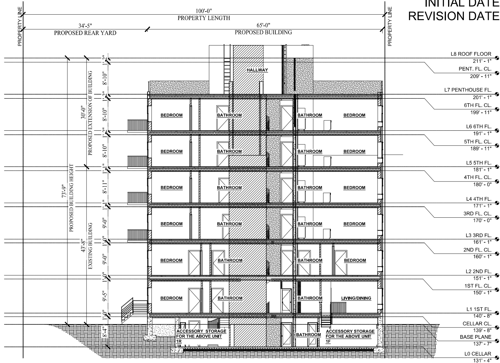
SECTION PLAN
