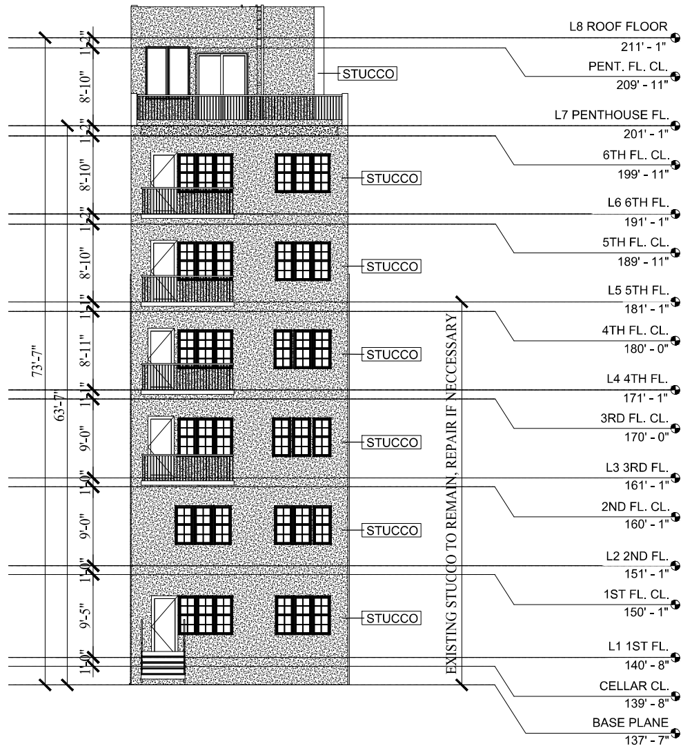
BACK ELEVATION (SOUTH)
