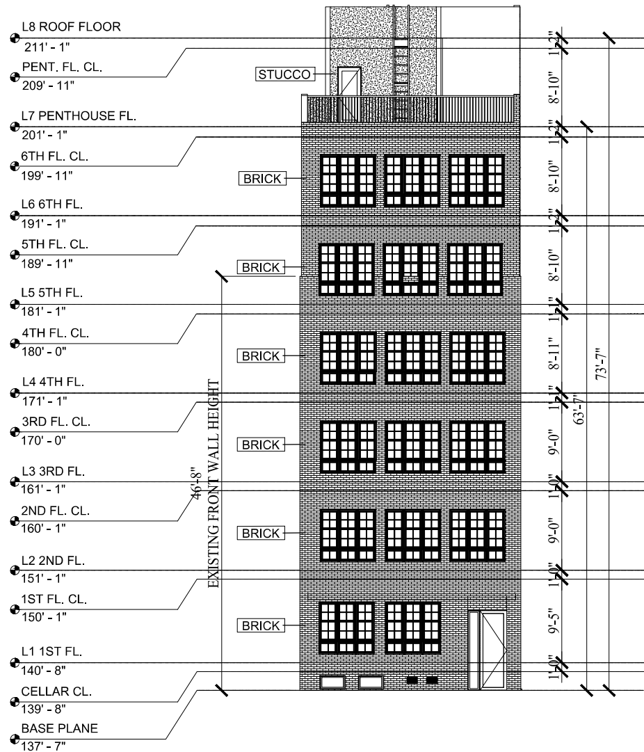
FRONT ELEVATION (NORTH)
