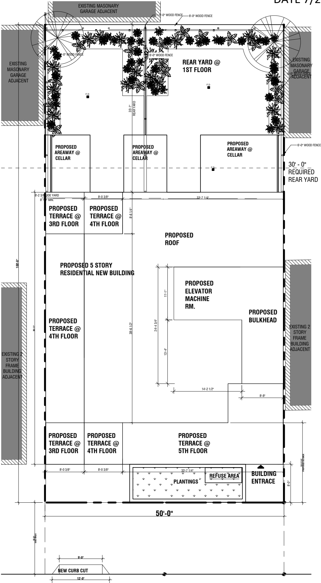
SITE PLAN
