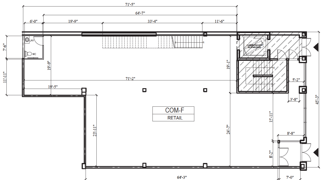
UNIT - COM-F (1st FLOOR INDOOR)
