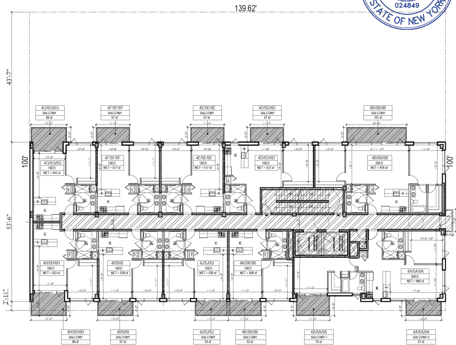
4th, 5th, 6th FLOOR PLAN
