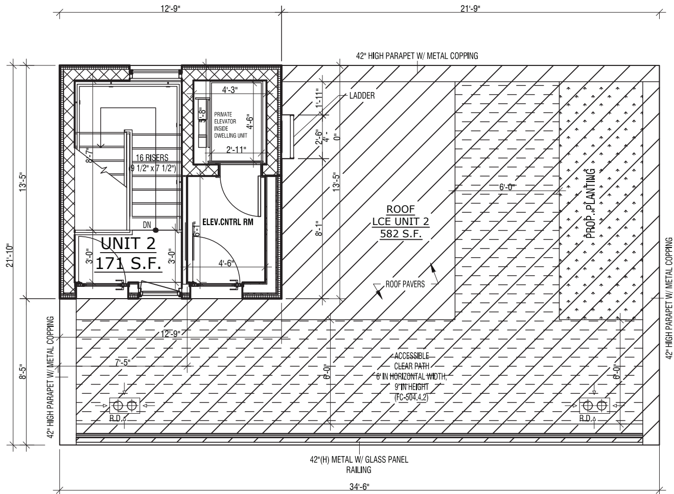
ROOF FLOOR PLAN
