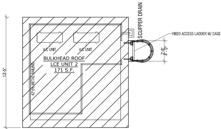
BULKHEAD ROOF FLOOR PLAN
