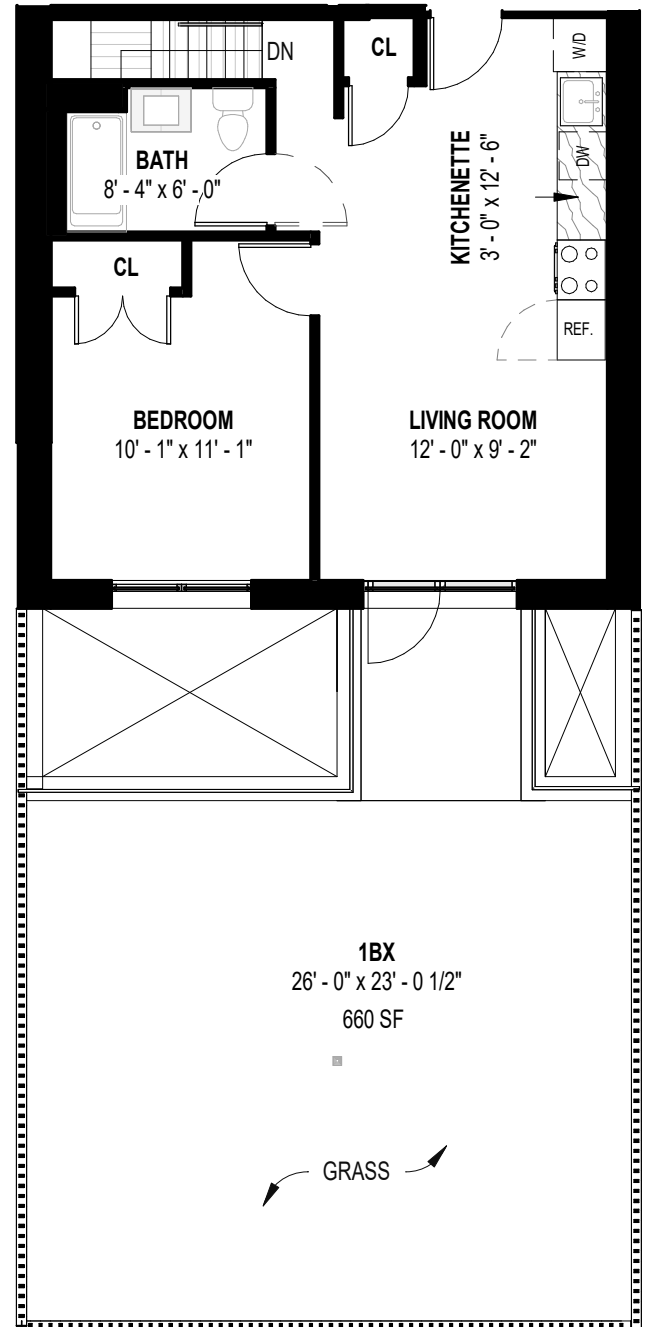
1ST FLOOR
