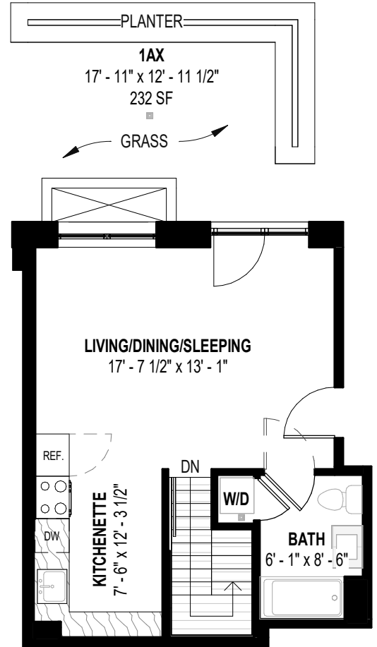
1ST FLOOR
