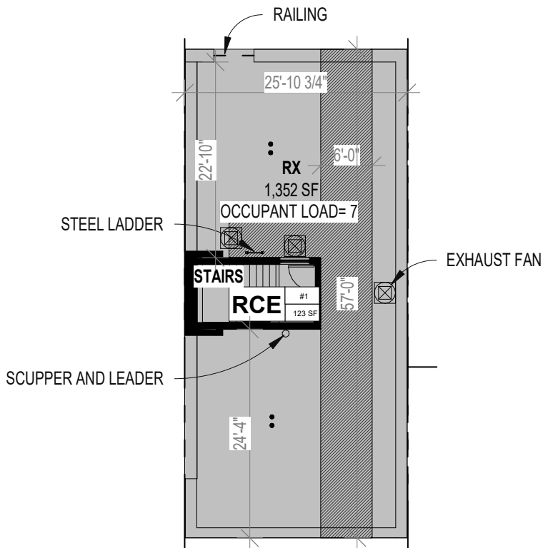
ROOF PLAN
