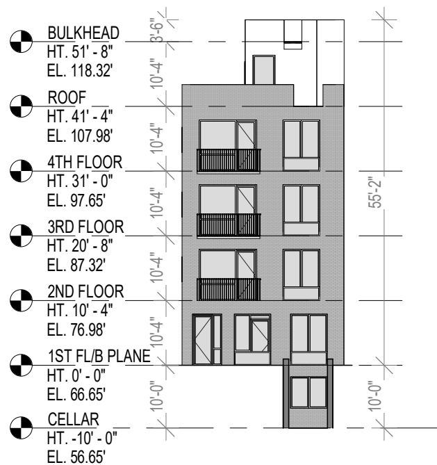
NORTHWEST ELEVATION
