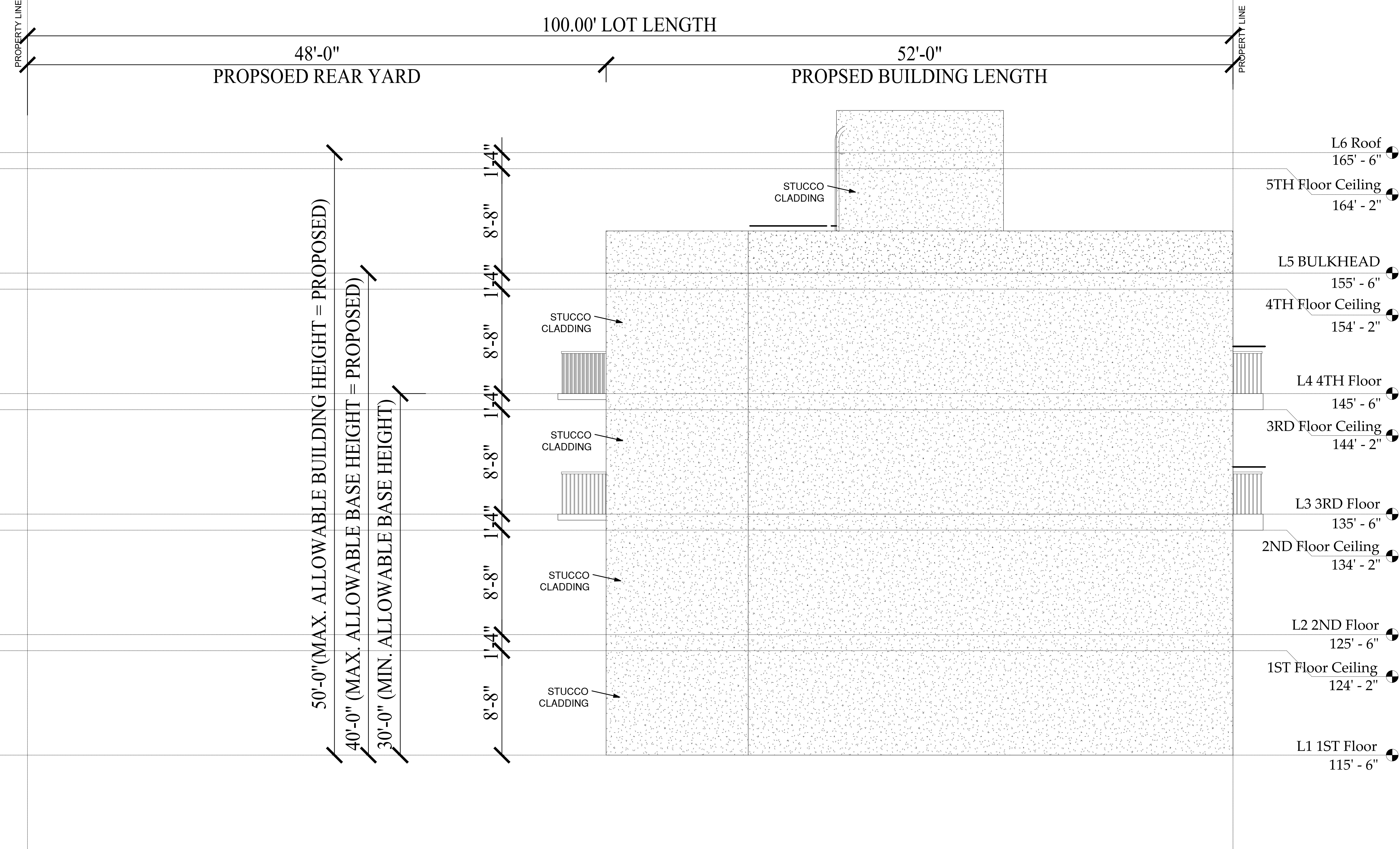
SIDE ELEVATION (WEST)
