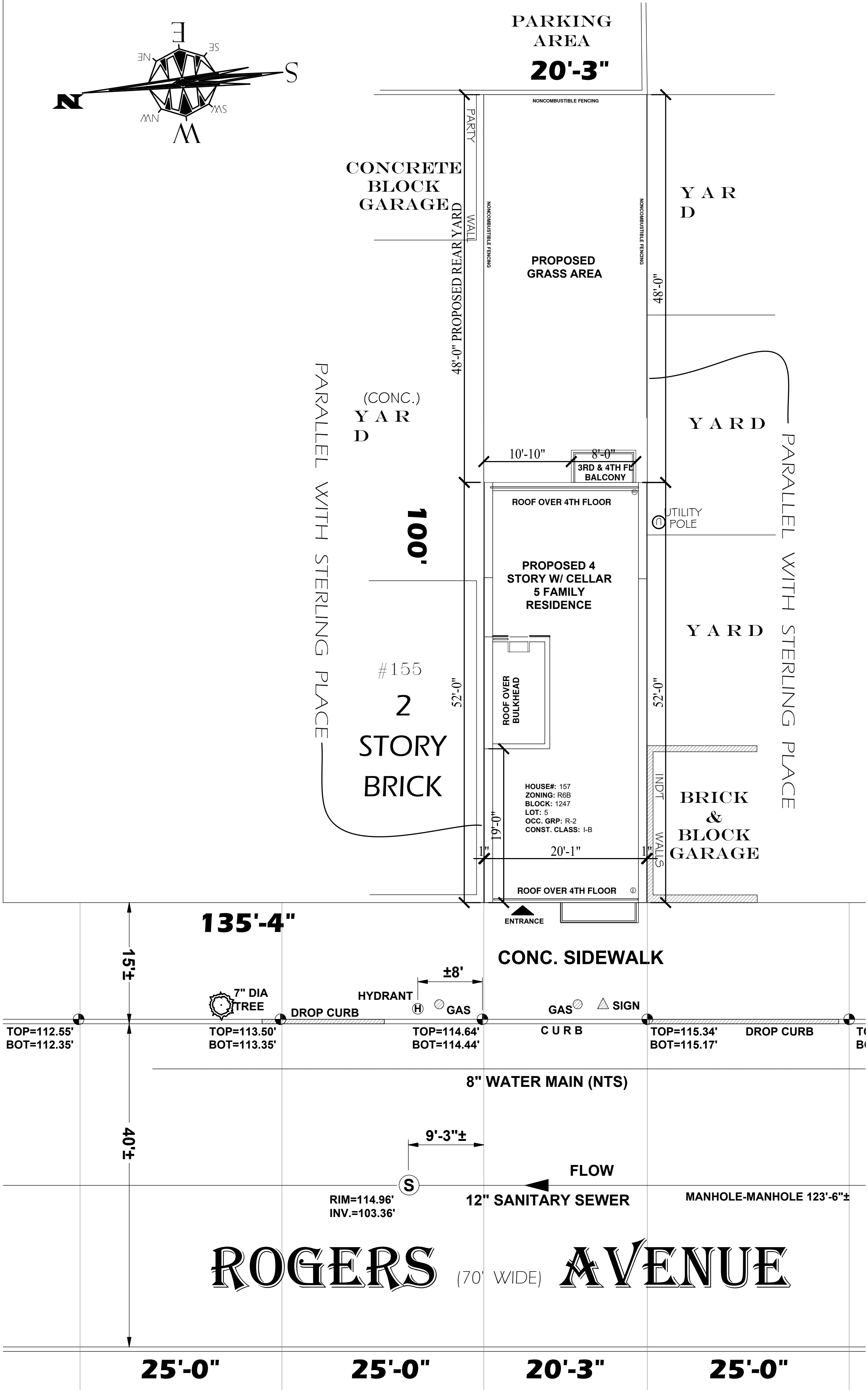
PLOT PLAN
