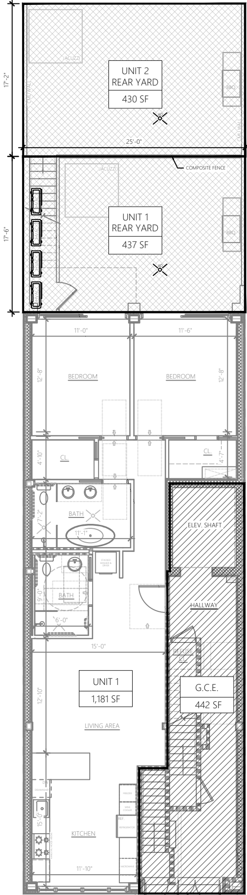
1st FLOOR PLAN SCALE: 3/32" = 1'-0"
