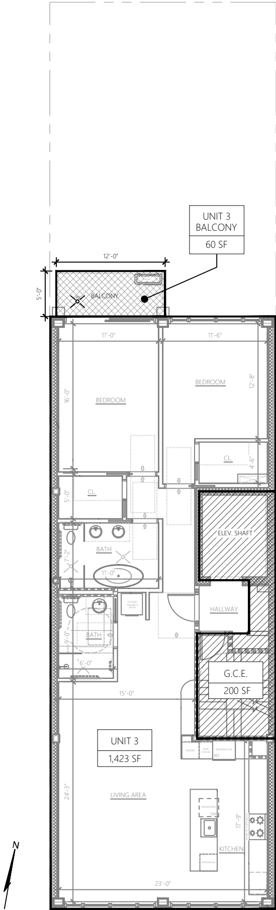
3rd FLOOR PLAN SCALE: 3/32" = 1'-0"
