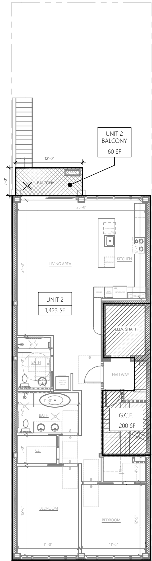
2nd FLOOR PLAN SCALE: 3/32" = 1'-0"
