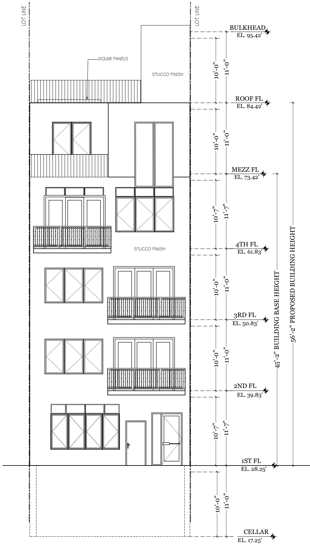
FRONT ELEVATION NOT SCALE
