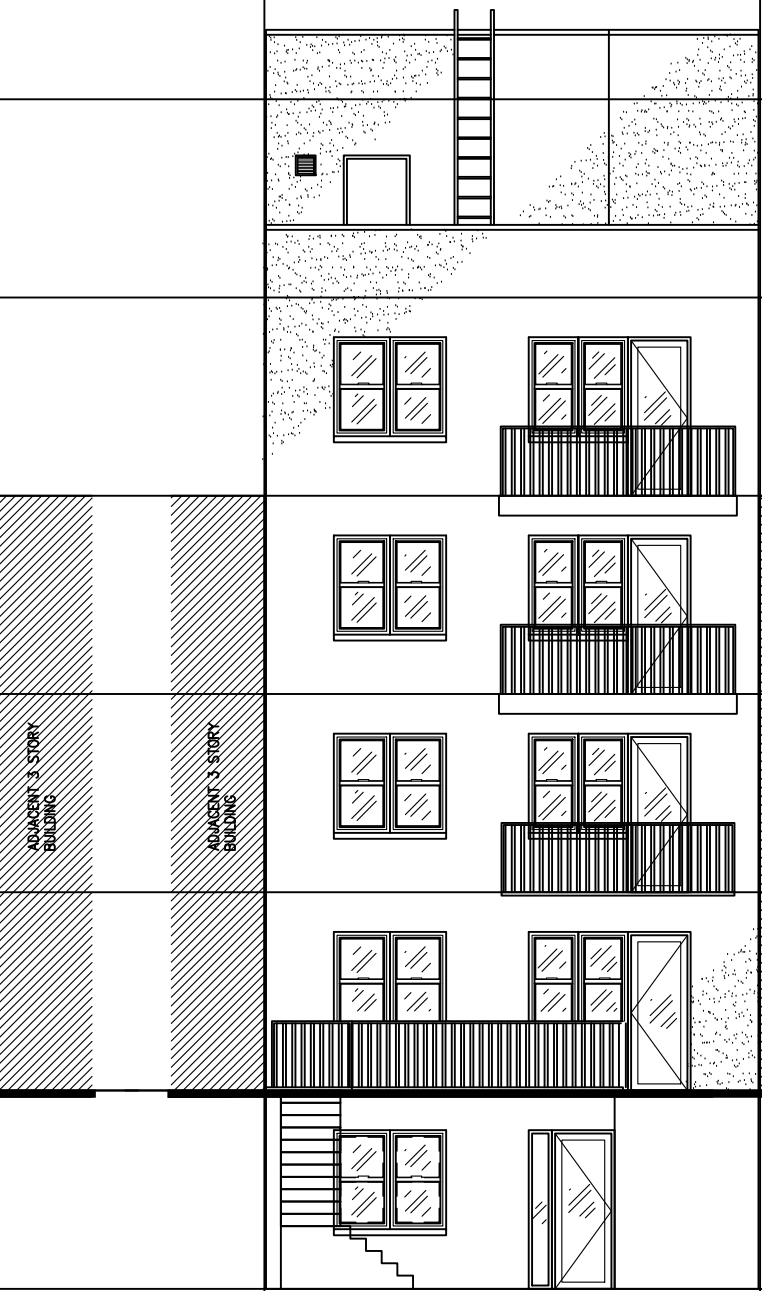
REAR ELEVATIONS
