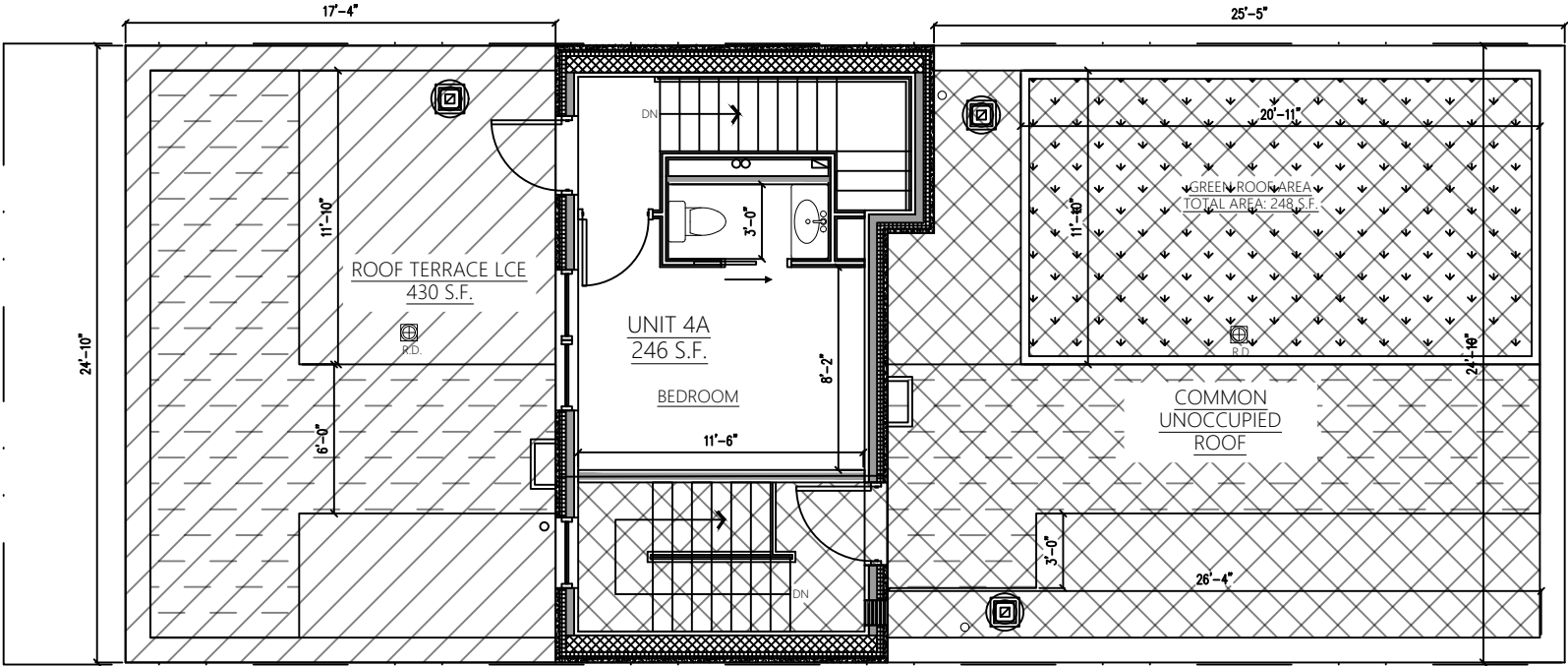
PENTHOUSE FLOOR PLAN
