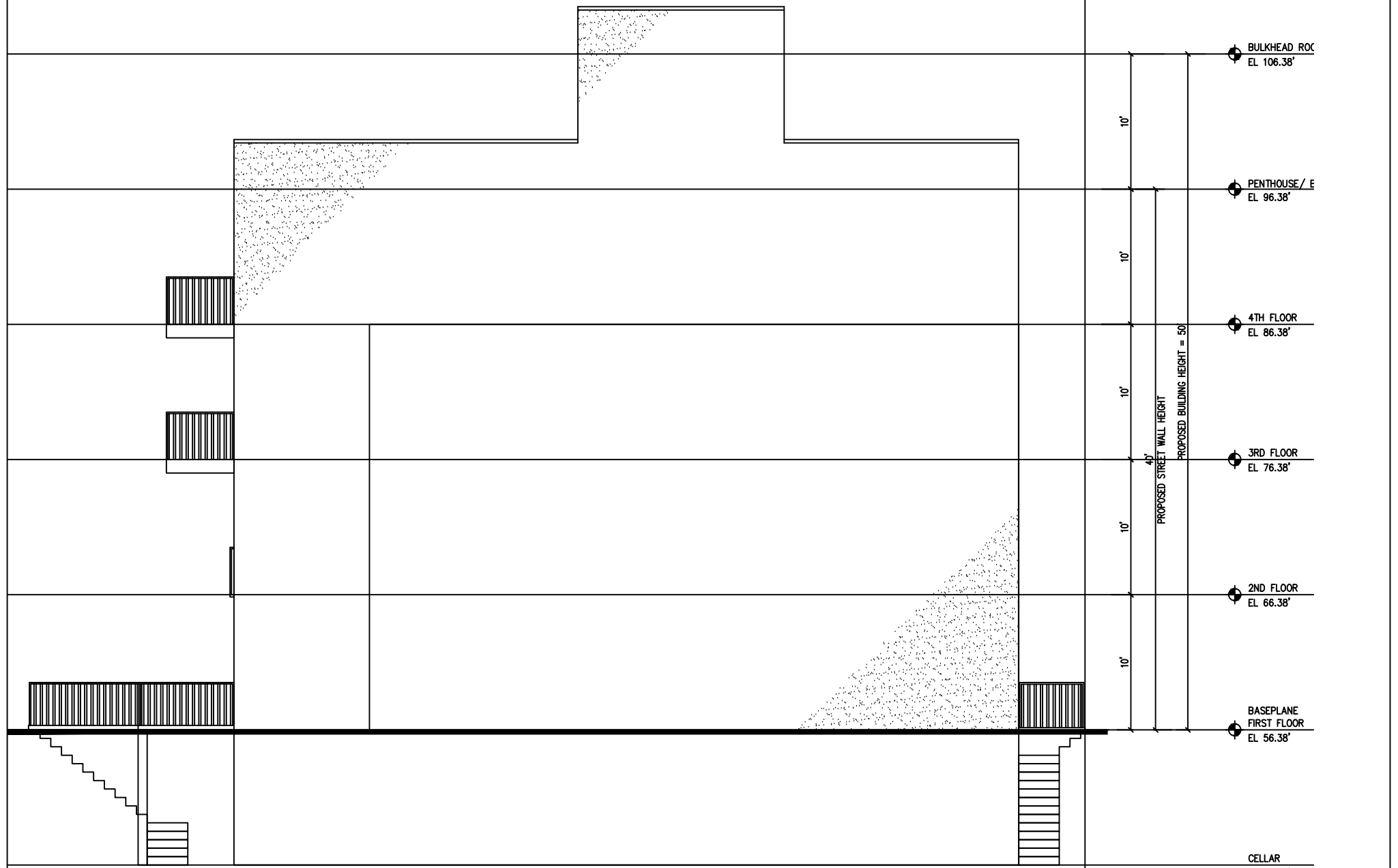
SIDE ELEVATIONS
