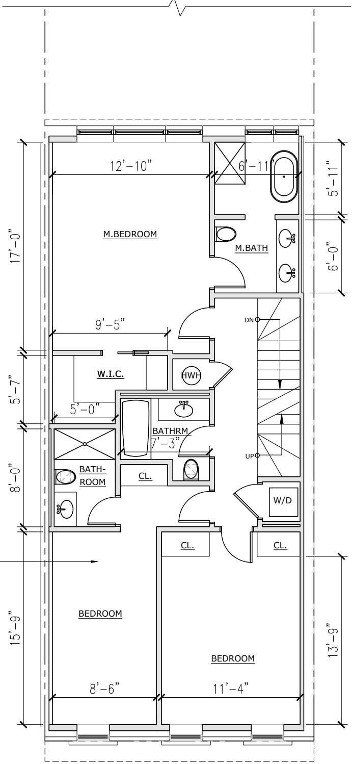
5 FOURTH FLOOR PLAN SCALE: 1/8"=1'-0"
