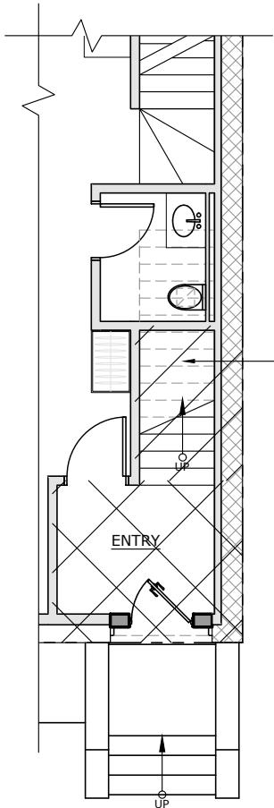
2 FIRST FLOOR PLAN (PARTIAL) SCALE: 1/8"=1'-0"
