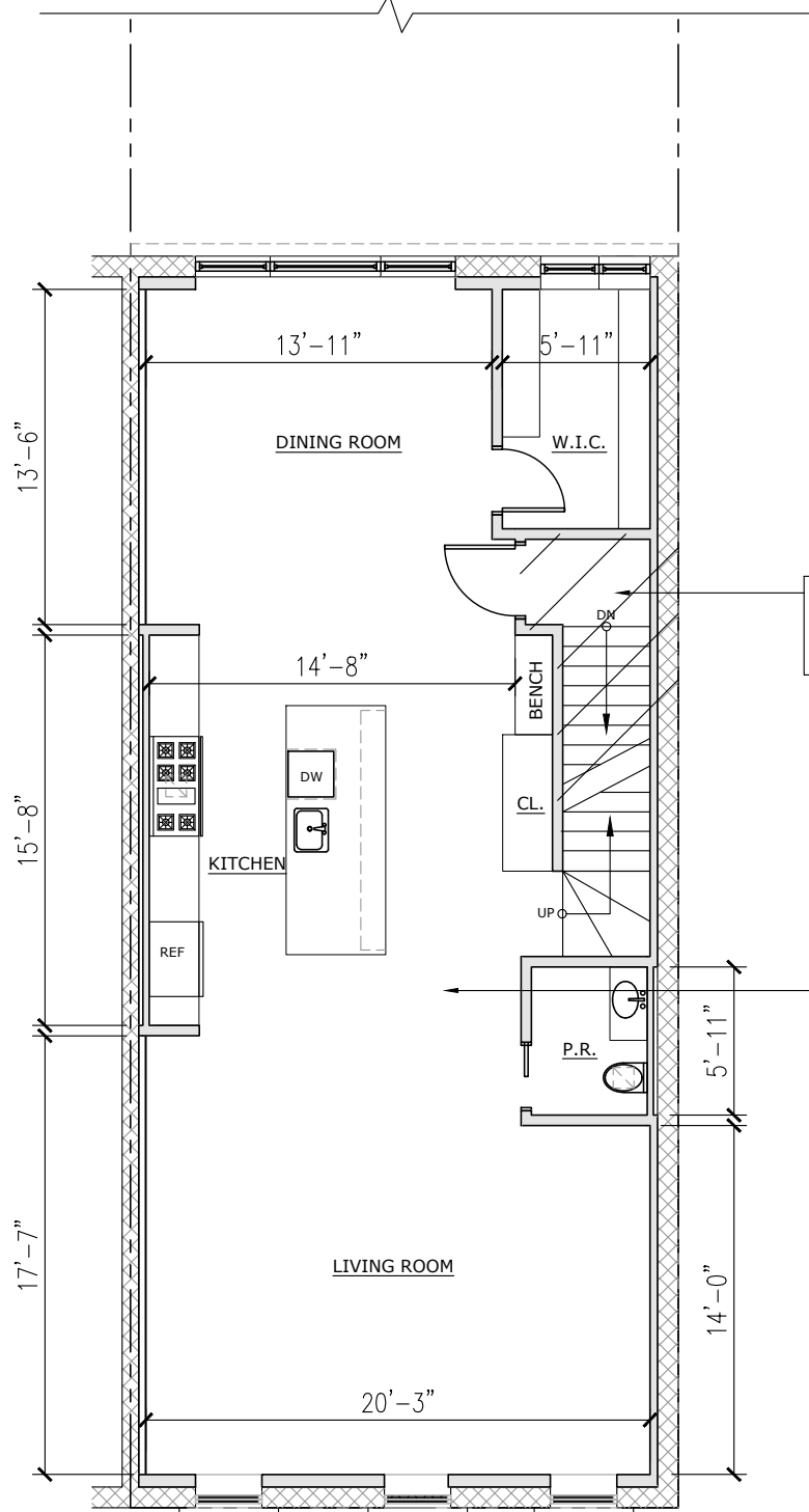
4 THIRD FLOOR PLAN SCALE: 1/8"=1'-0"
