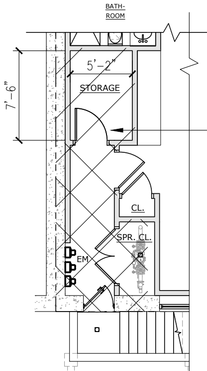
1 CELLAR FLOOR PLAN (PARTIAL) SCALE: 1/8"=1'-0"
