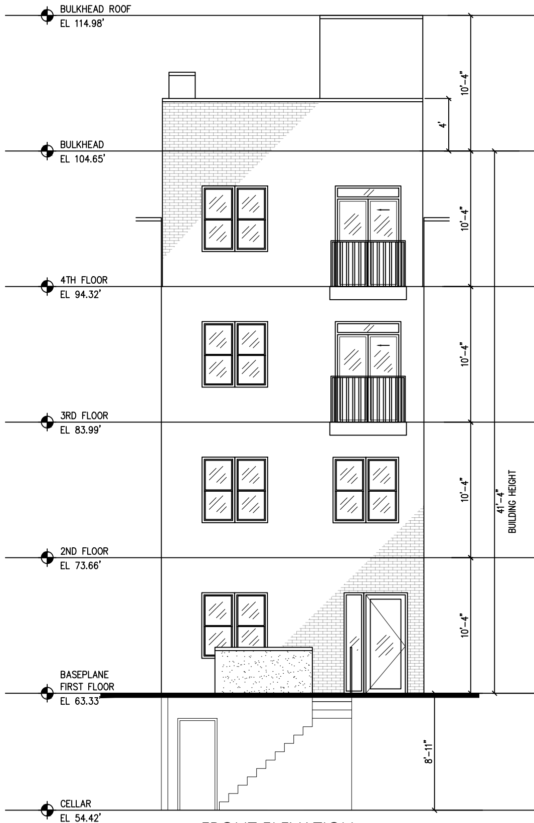
FRONT ELEVATION
