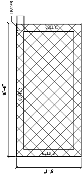
BULKHEAD FLOOR PLAN
