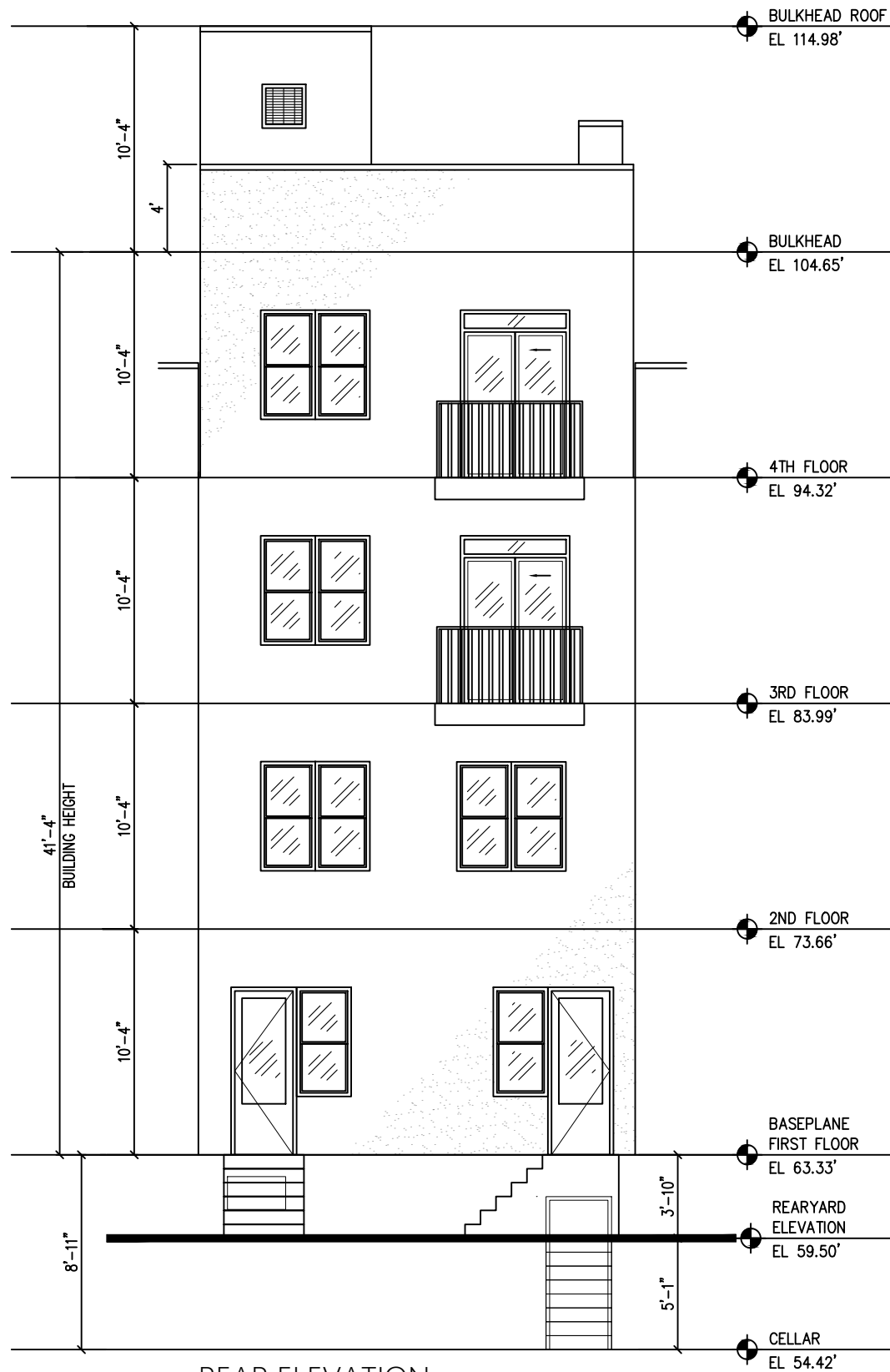
REAR ELEVATION
