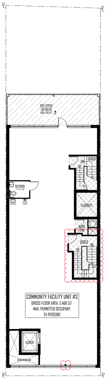
41st ROAD 2nd FLOOR PLAN SCALE : 1/16" = 1'-0"
