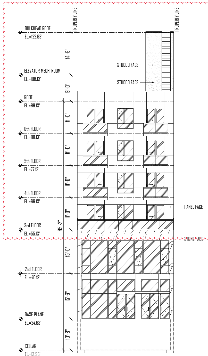
41st ROAD FRONT ELEVATION SCALE: 1/16" = 1'-0"
