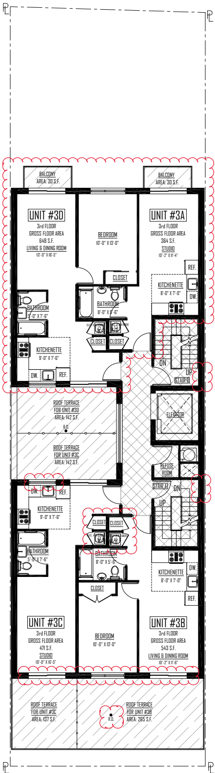
41st ROAD 3rd FLOOR PLAN SCALE : 1/16" = 1'-0"
