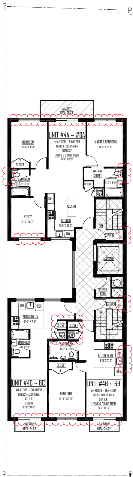
41st ROAD 4th ~ 6th FLOOR PLAN SCALE : 1/16" = 1'-0"
