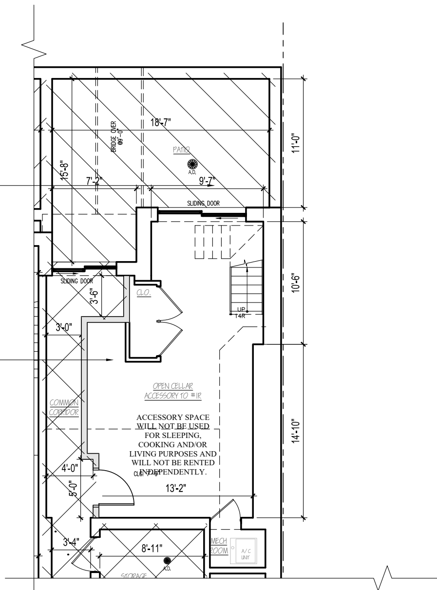
CELLAR FLOOR PLAN (PARTIAL) SCALE: 1/8"=1'-0"
