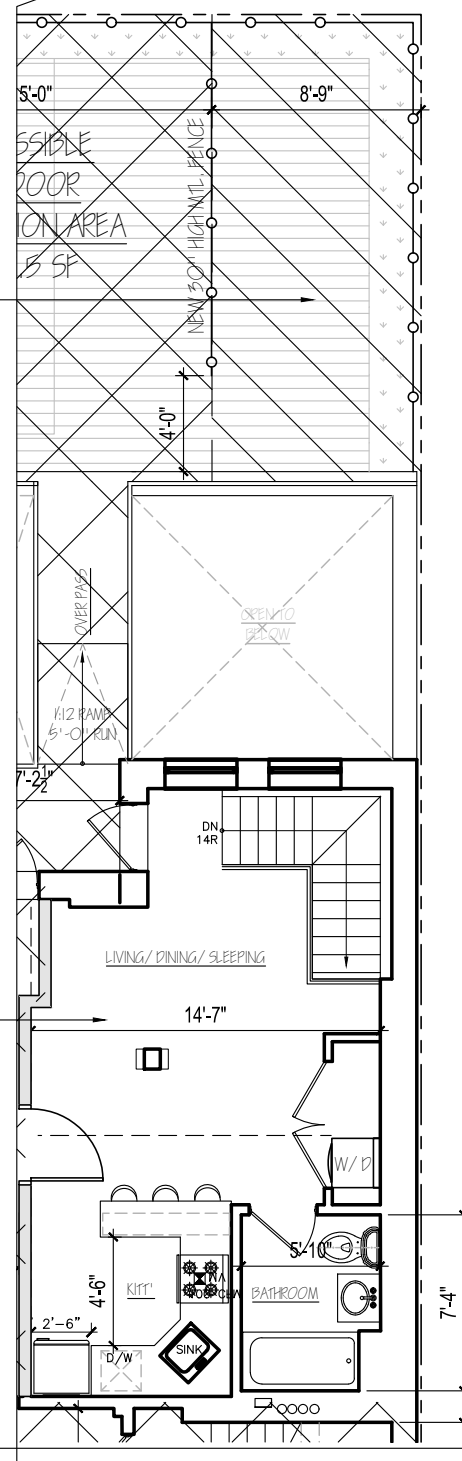
BASEMENT FLOOR PLAN (PARTIAL) SCALE: 1/8"=1'-0"
