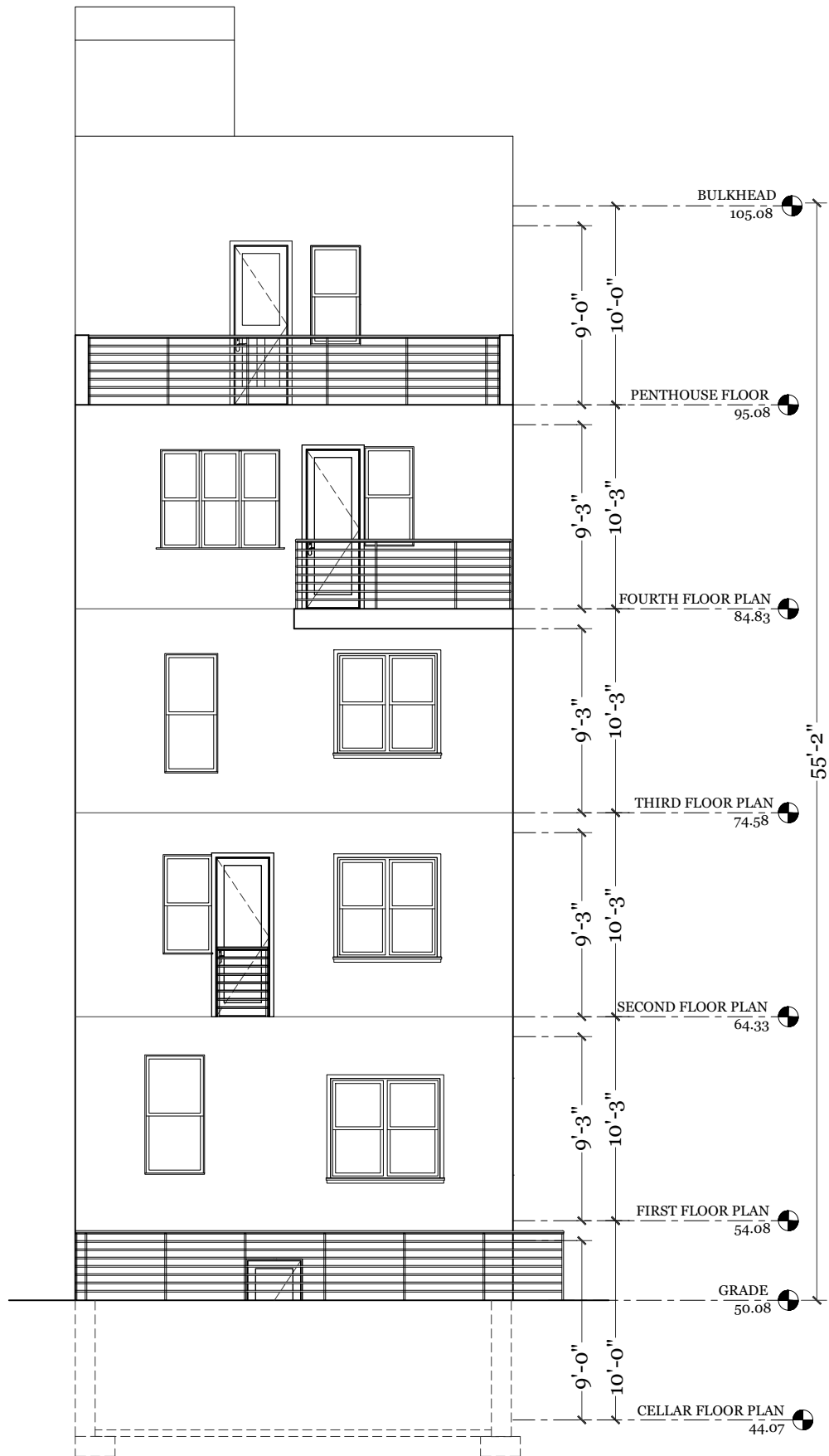
REAR ELEVATION SCALE 1/8" = 1'-0"
