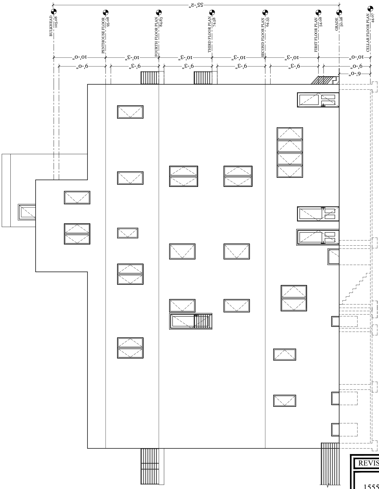
LEFT ELEVATION NOT SCALE
