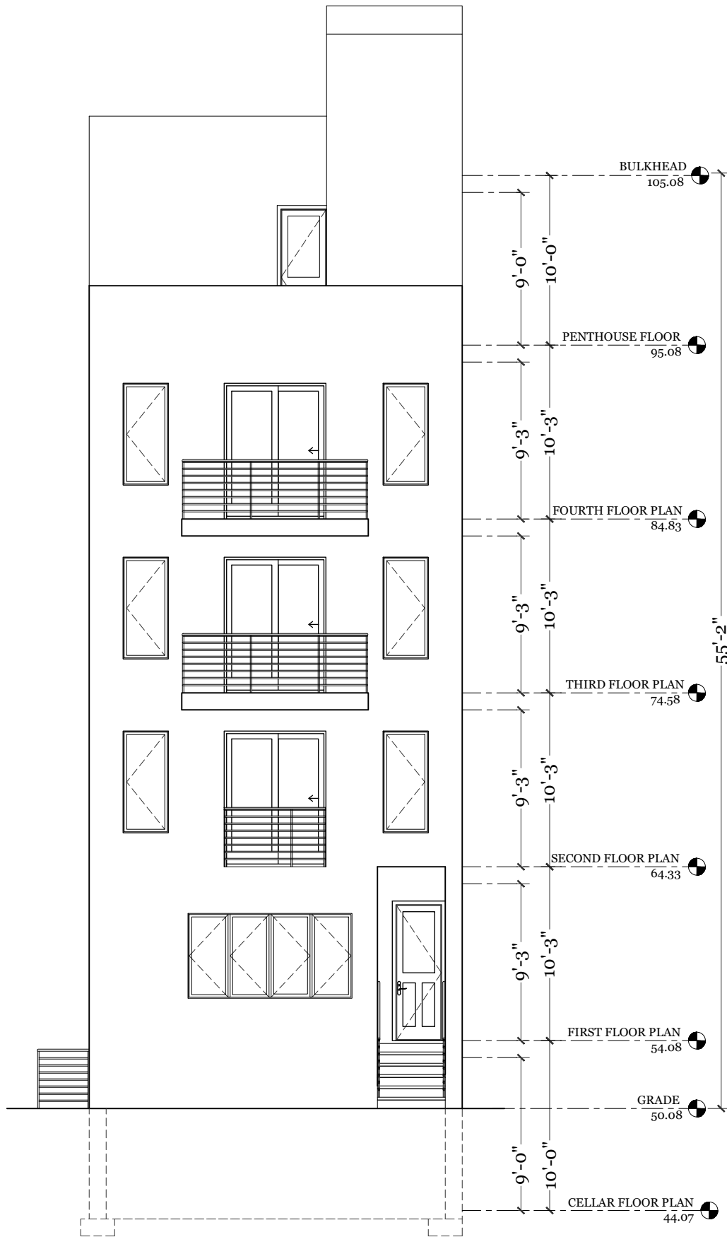
FRONT ELEVATION SCALE 1/8" = 1'-0"
