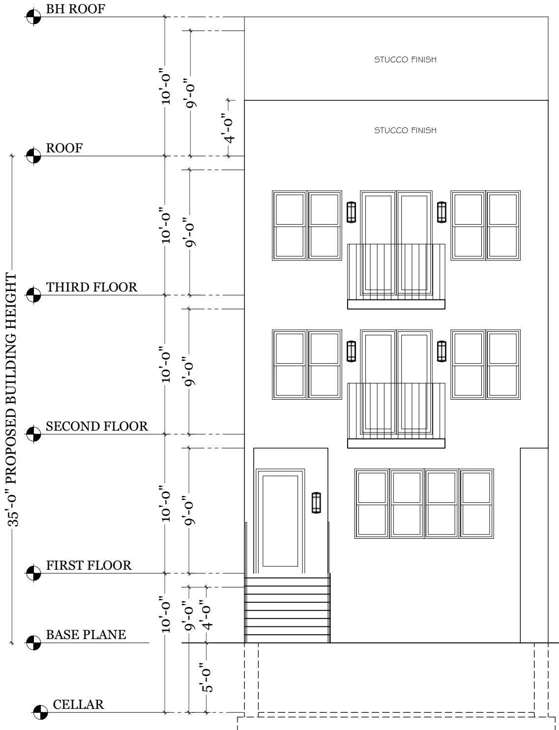
FRONT ELEVATION NOT SCALE
