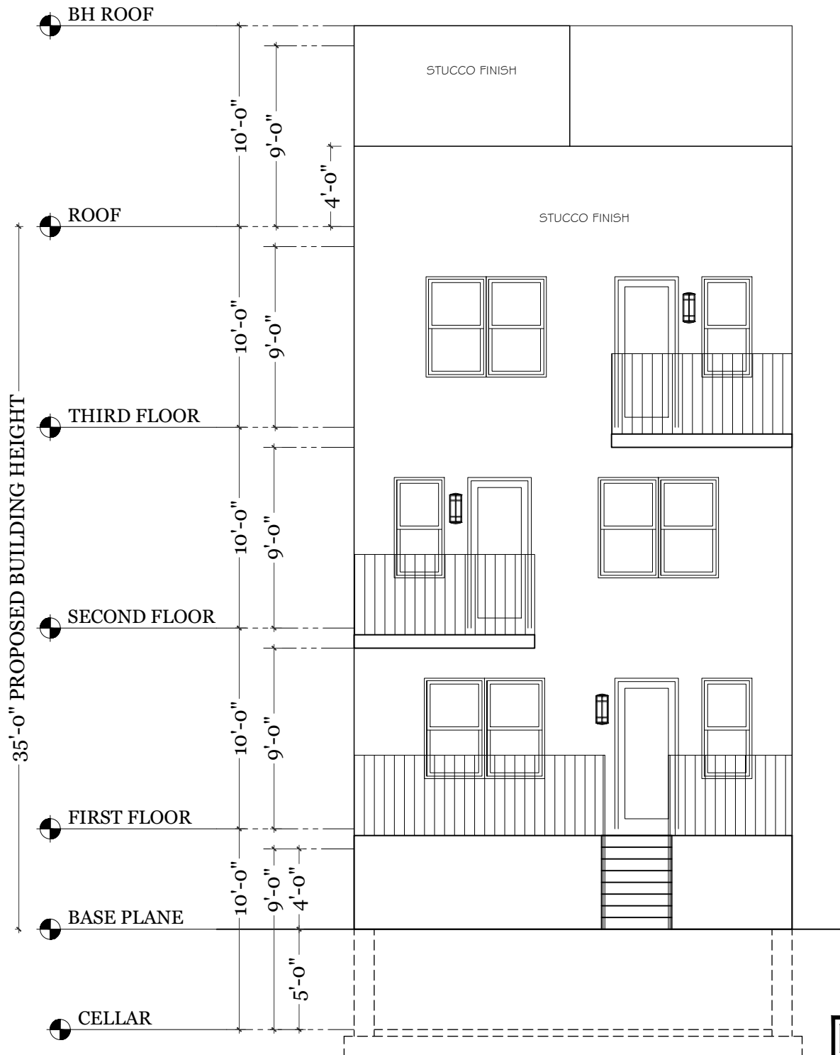
REAR ELEVATION NOT SCALE
