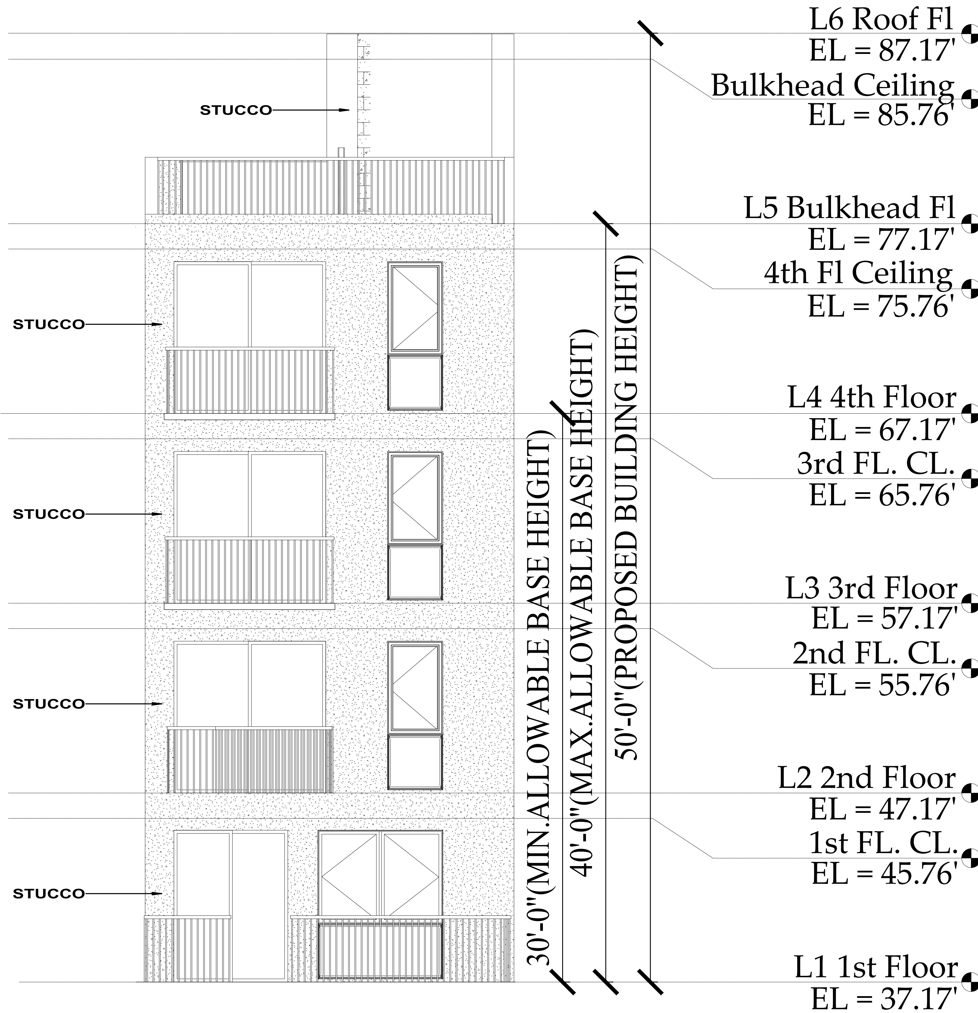
BACK ELEVATION (NORTH)
