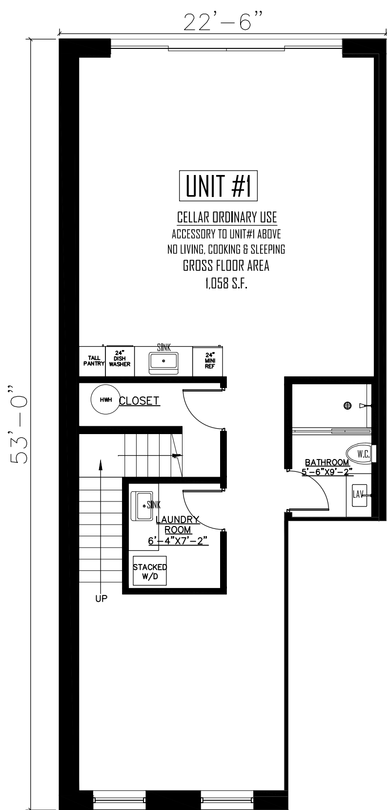
CELLAR FLOOR PLAN
