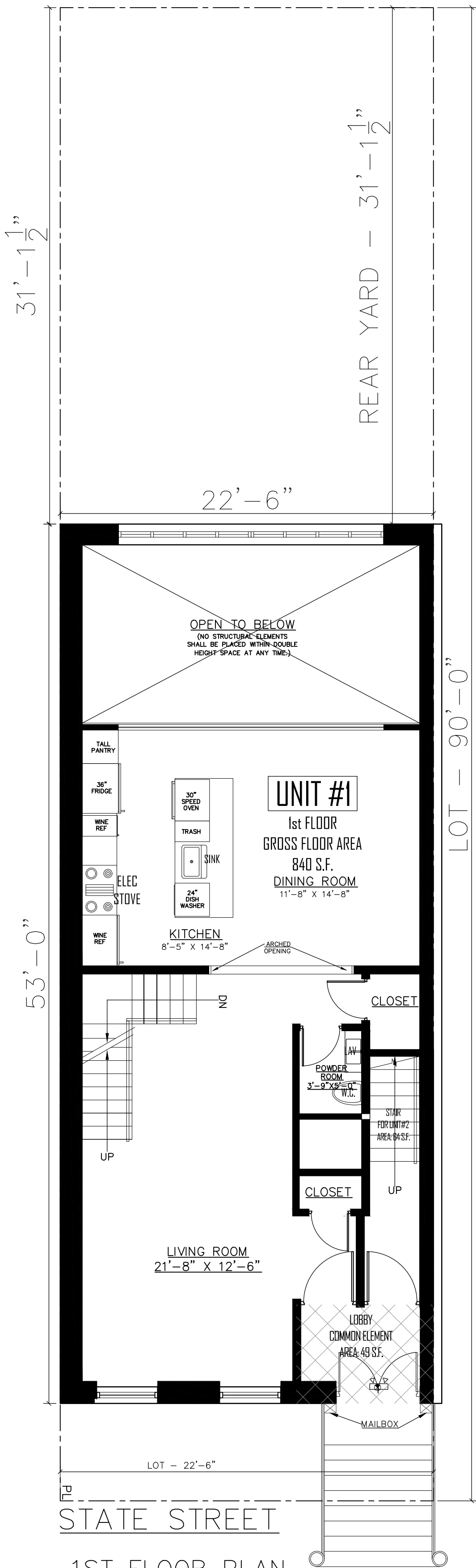
1ST FLOOR PLAN SCALE: 3/8" = 1'-0"
