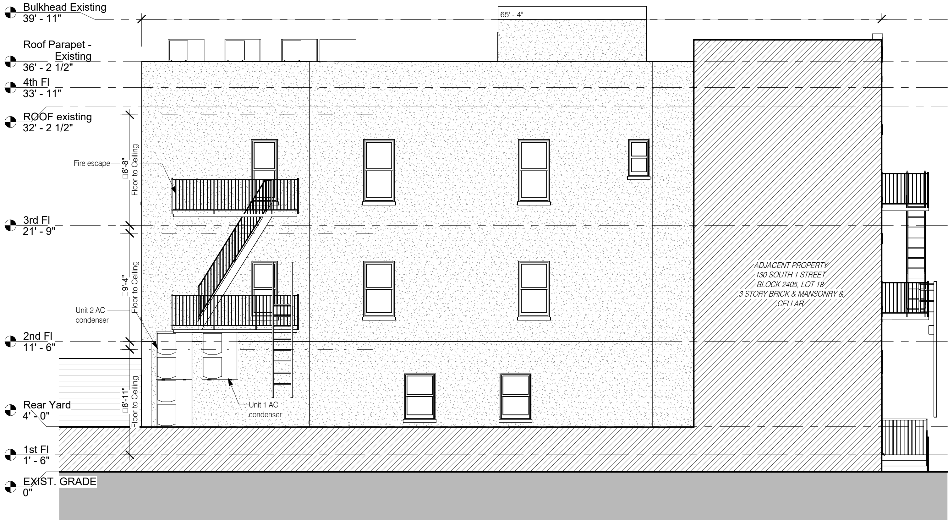
SIDE ELEVATION OP-9 10/9/25 REV 12/8/2025
