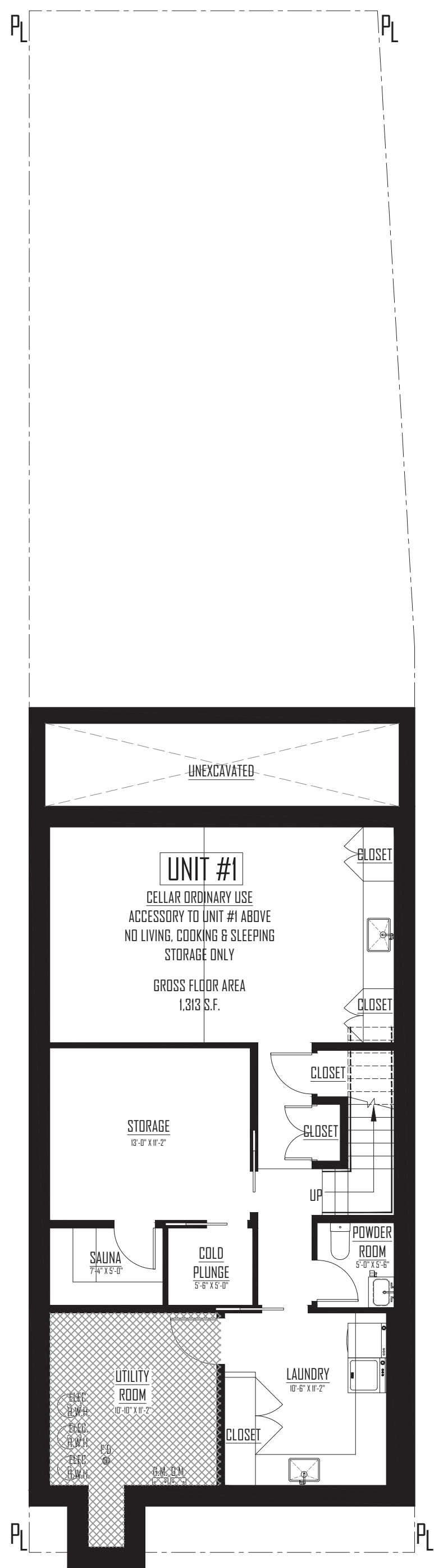
BALTIC STREET CELLAR PLAN SCALE: 3/40"=1'-0"
