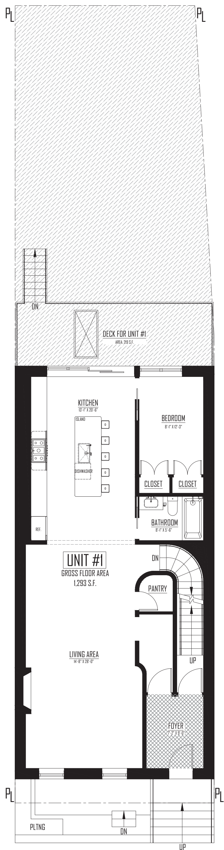
BALTIC STREET 1st FLOOR PLAN SCALE: 3/40"= 1'-0"
