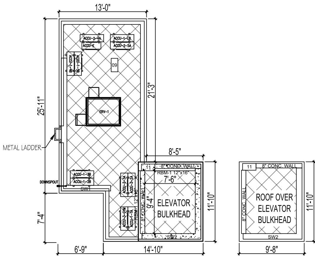
BULKHEAD ROOF FLOOR PLAN
