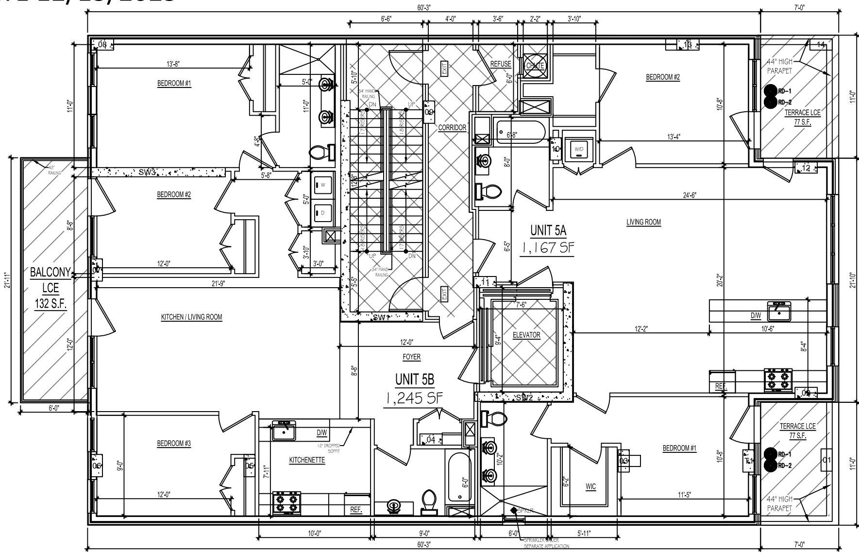
FIFTH FLOOR PLAN
