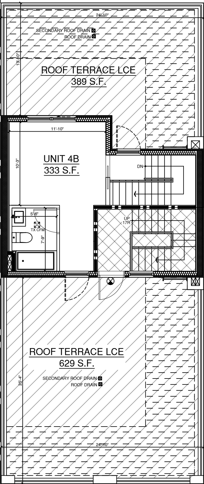
PENTHOUSE FLOOR PLAN
