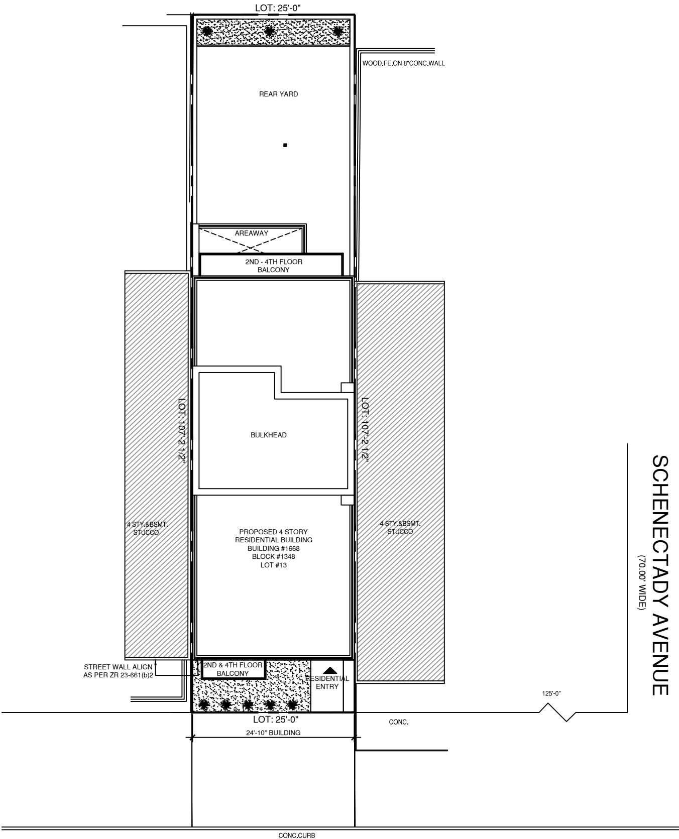
SITE PLAN
