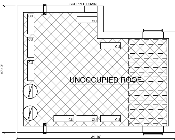
BULKHEAD FLOOR PLAN
