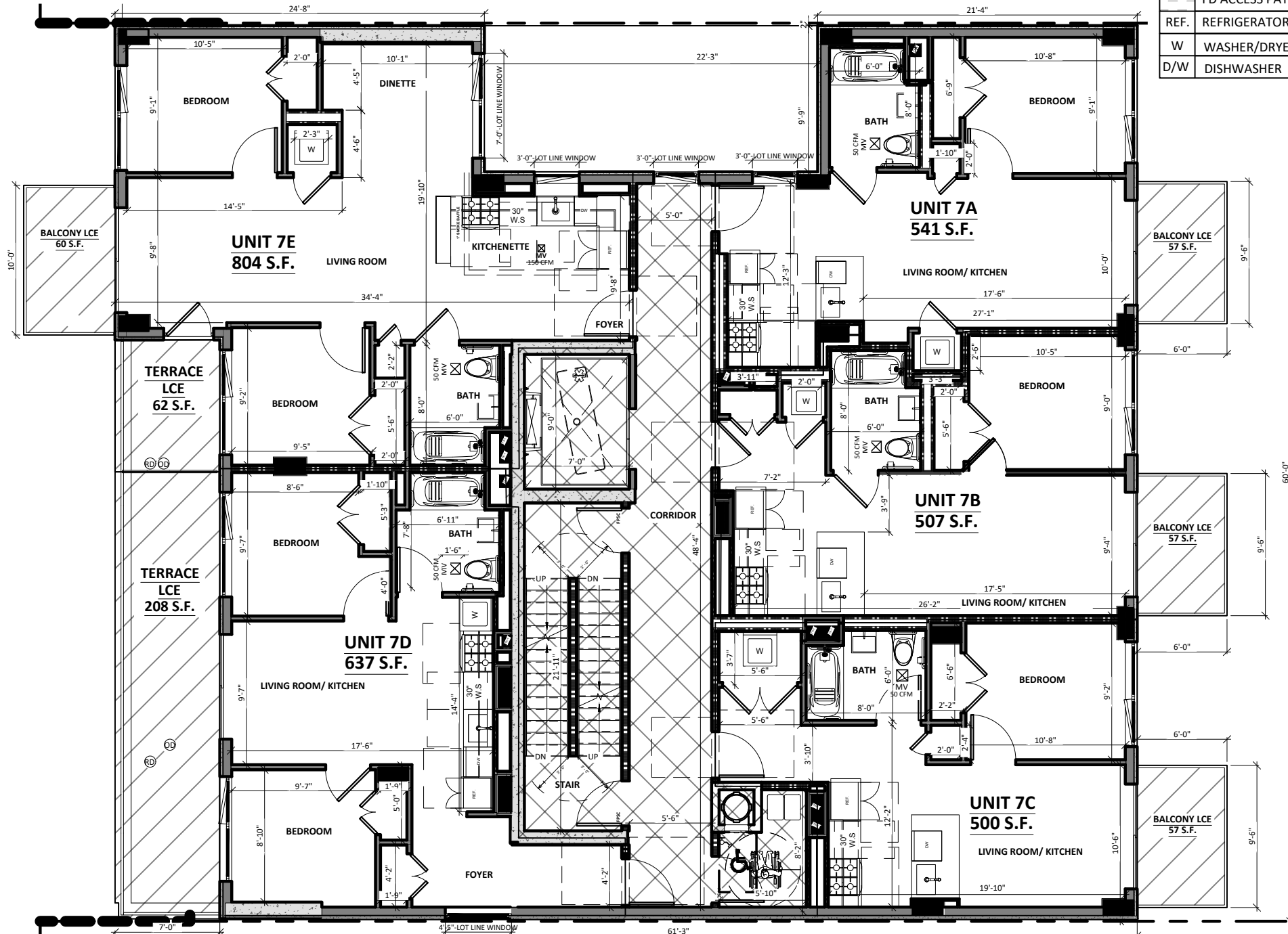
7TH FLOOR PLAN
