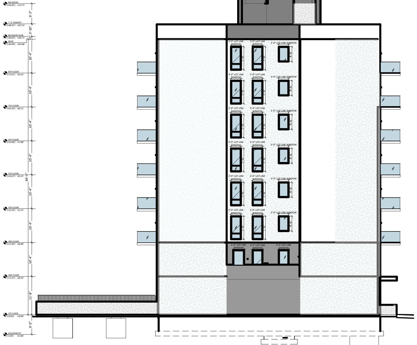
NORTH ELEVATION
