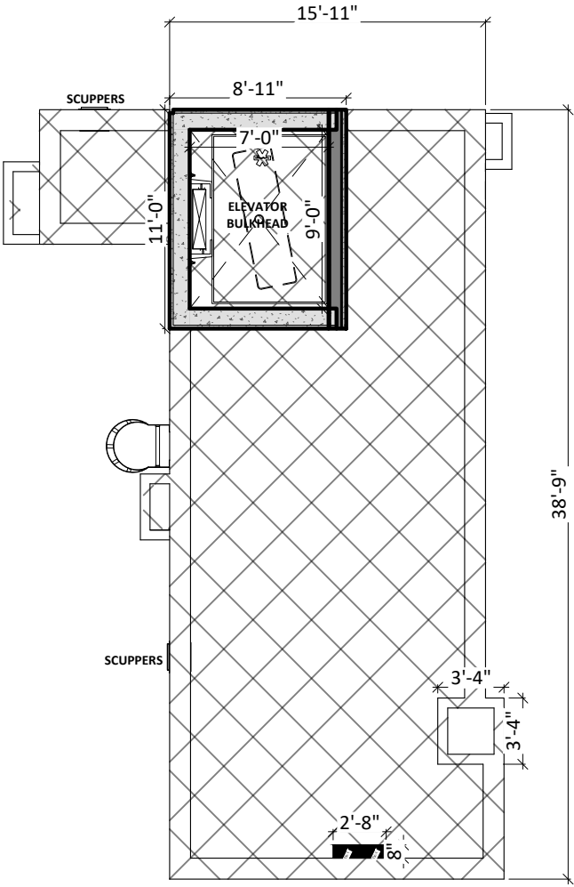
ROOF BULKHEAD PLAN
