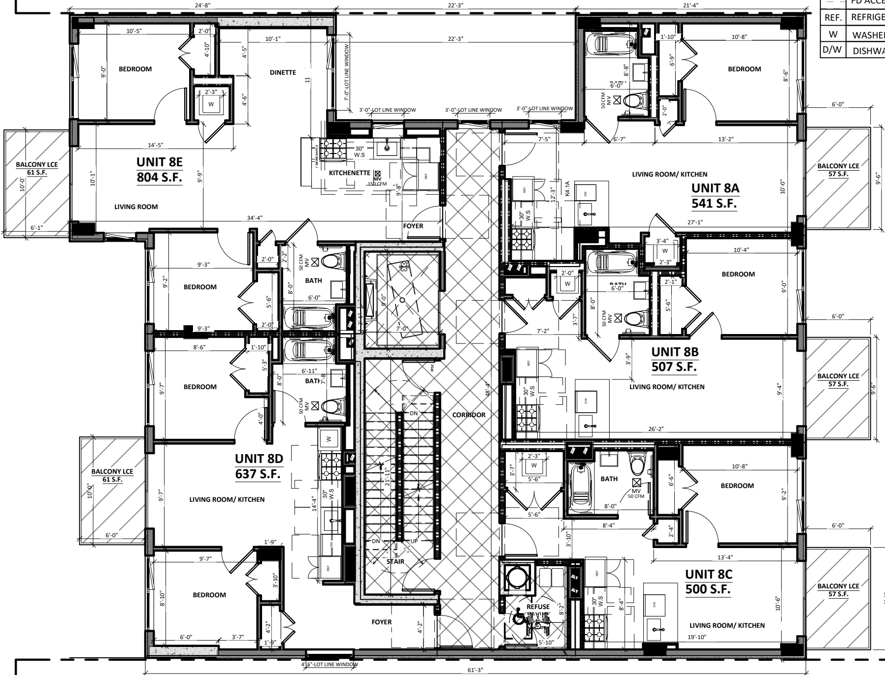
8TH FLOOR PLAN
