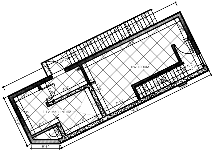
BULKHEAD FLOOR PLAN
