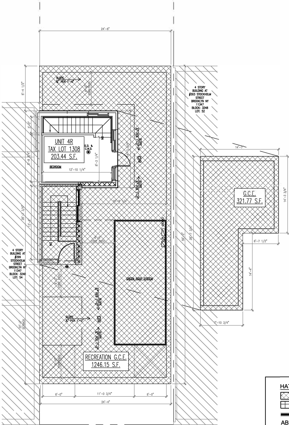
ROOF FLOOR PLAN Scale: 3/32" = 1'-0"
