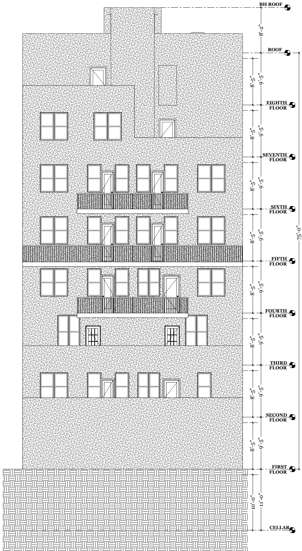
REAR ELEVATION SCALE 3/32" = 1'-0"
