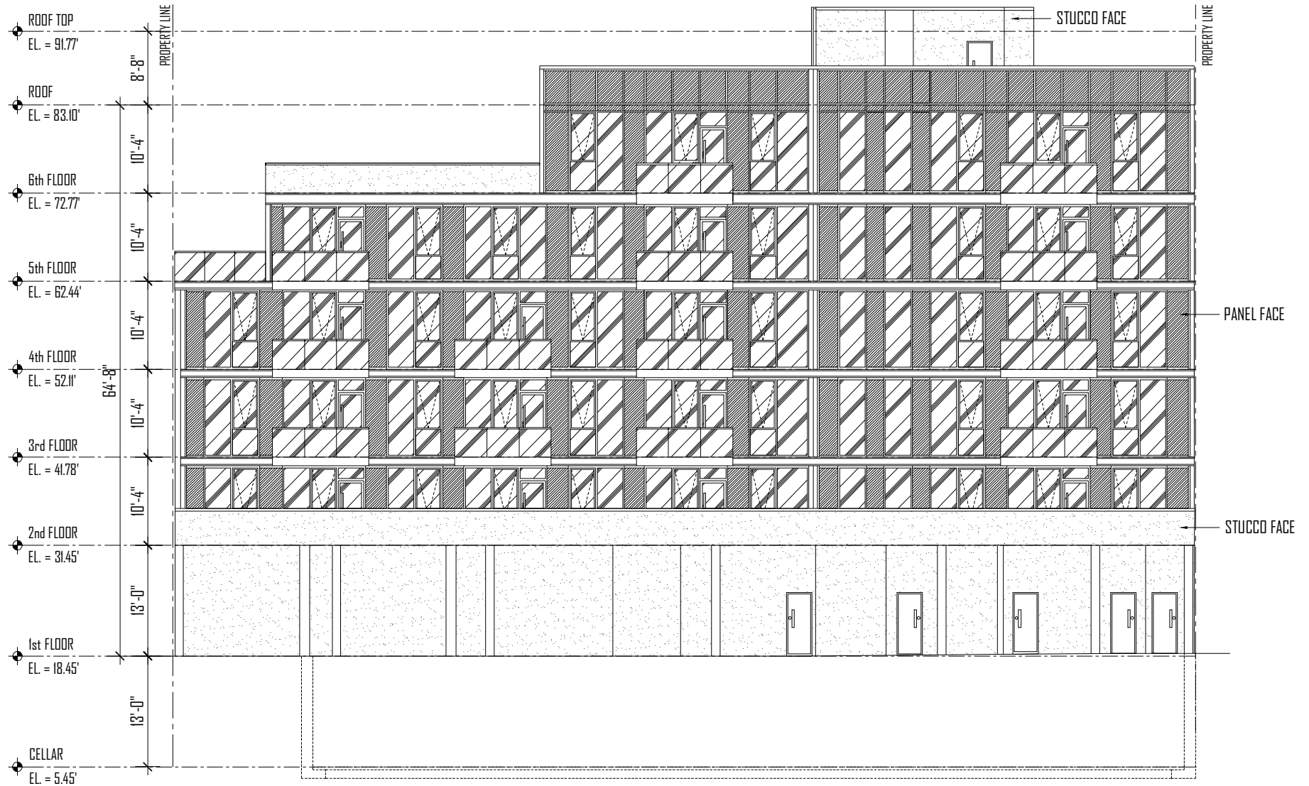
NORTH ELEVATION SCALE: 1/16"=1'-0"
