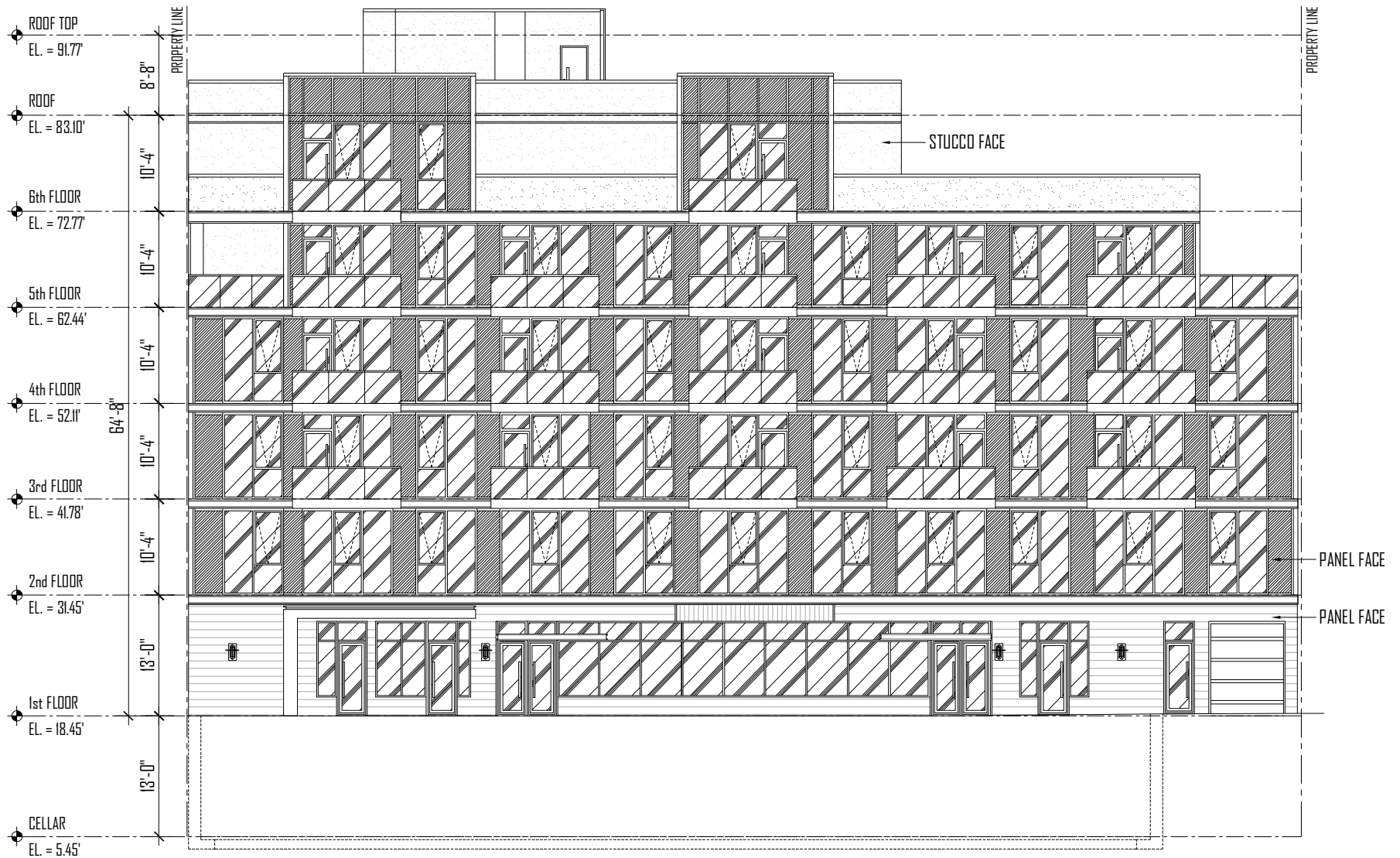
49th AVENUE SOUTH ELEVATION SCALE: 1/16"=1'-0"
