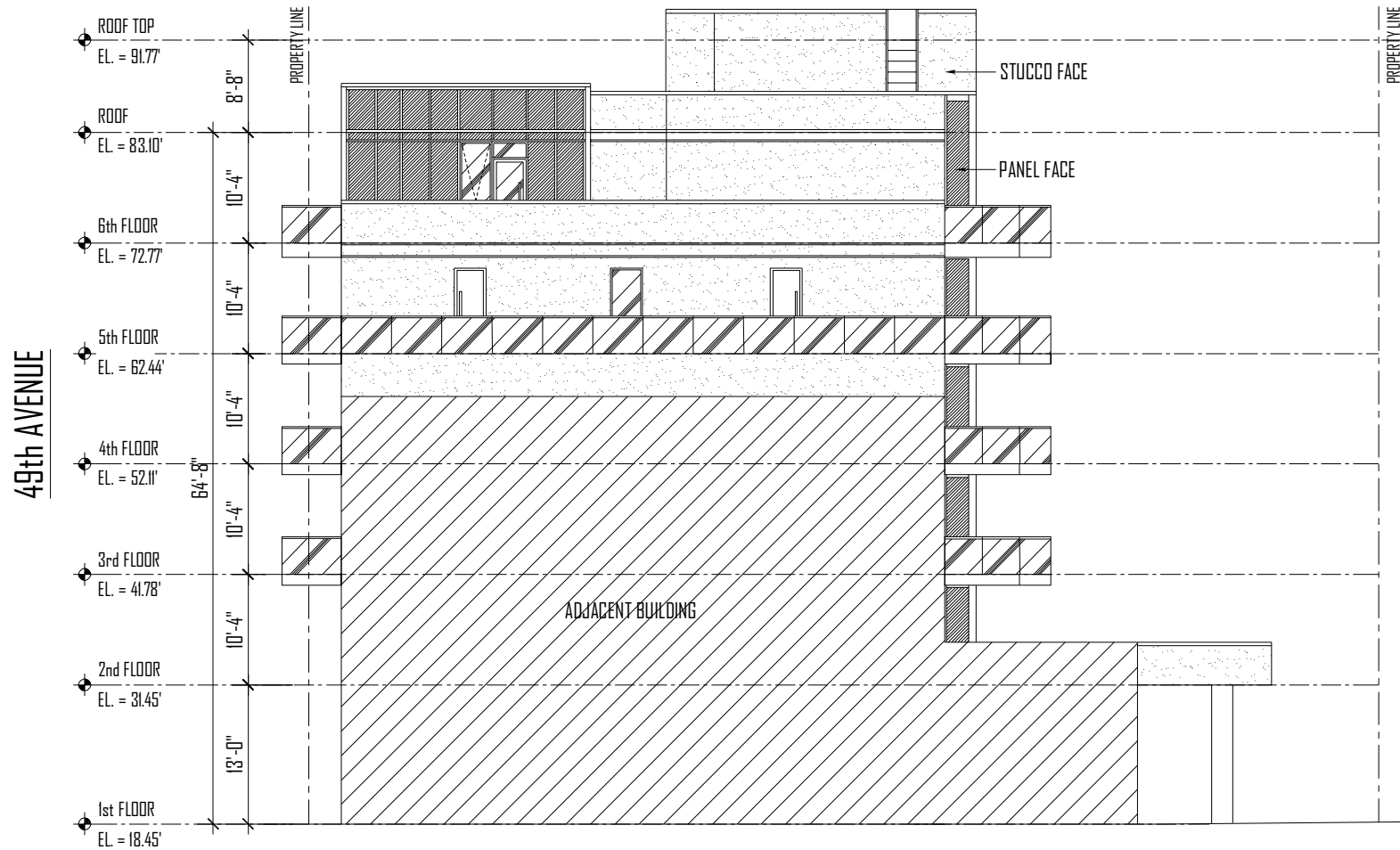
EAST ELEVATION SCALE: 1/16"=1'-0"
