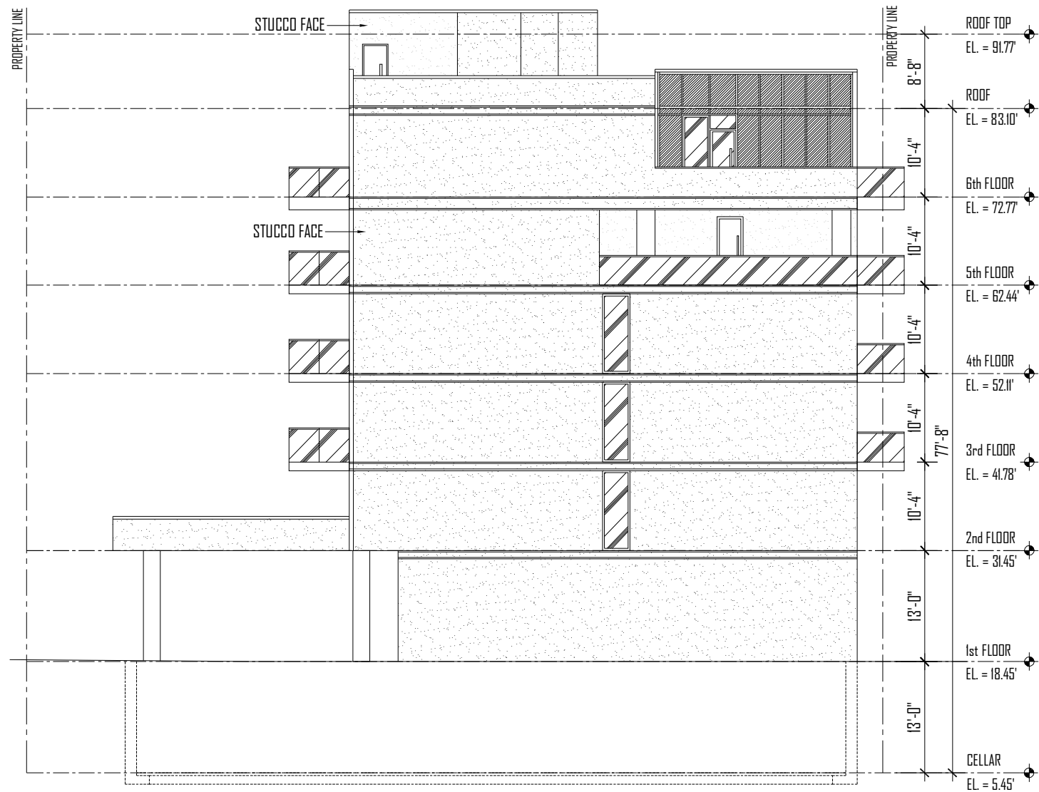
WEST ELEVATION SCALE: 1/16"=1'-0"
