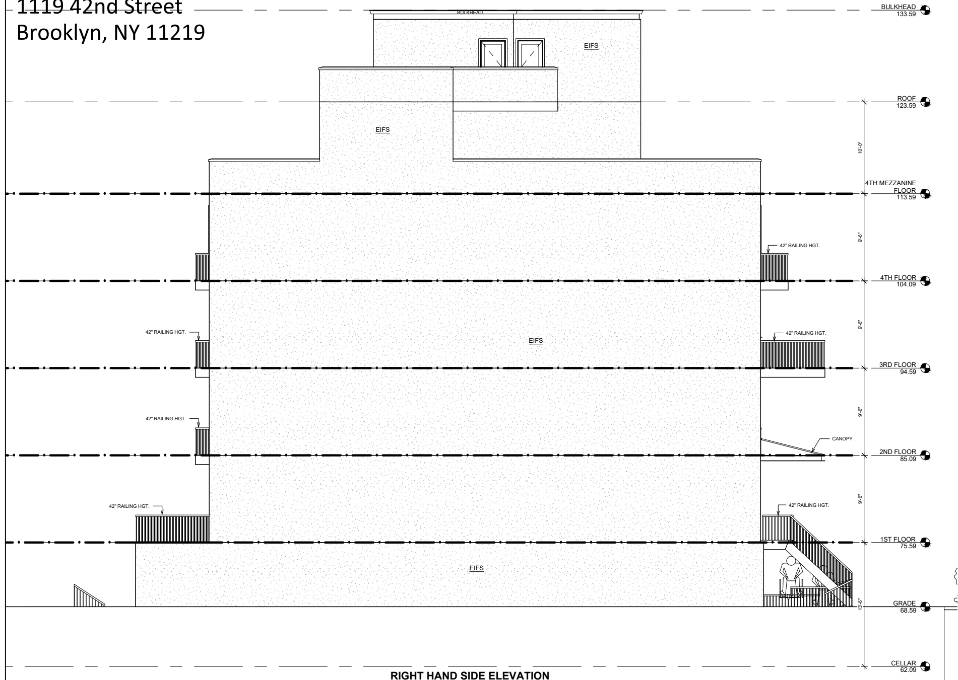
RIGHT HAND SIDE ELEVATION
