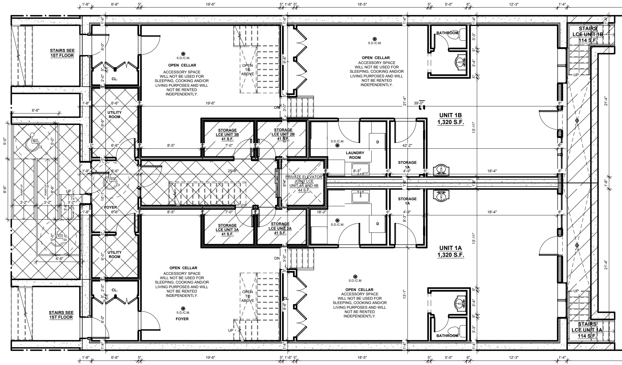
CELLAR FLOOR PLAN
