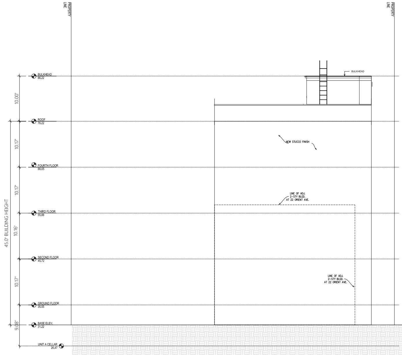
WEST ELEVATION
