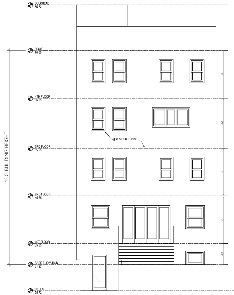
REAR ELEVATION
