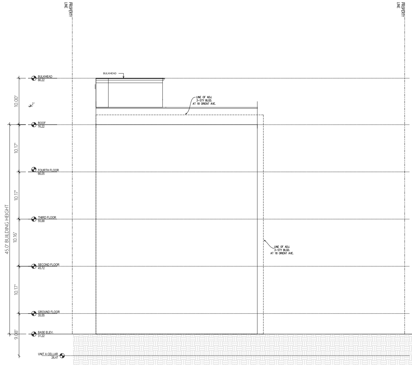
EAST ELEVATION
