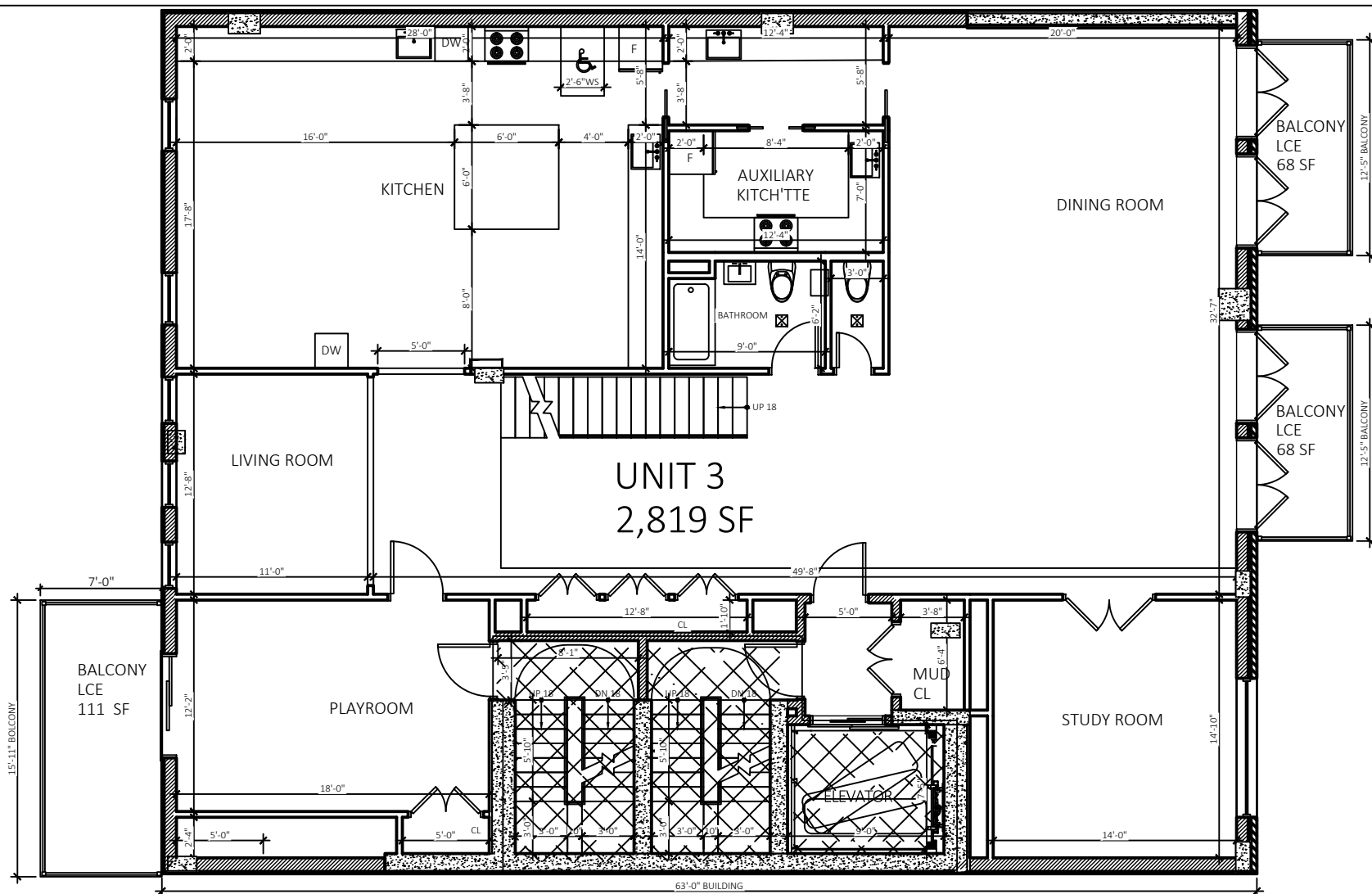
5TH FLOOR PLAN-UNIT 3
