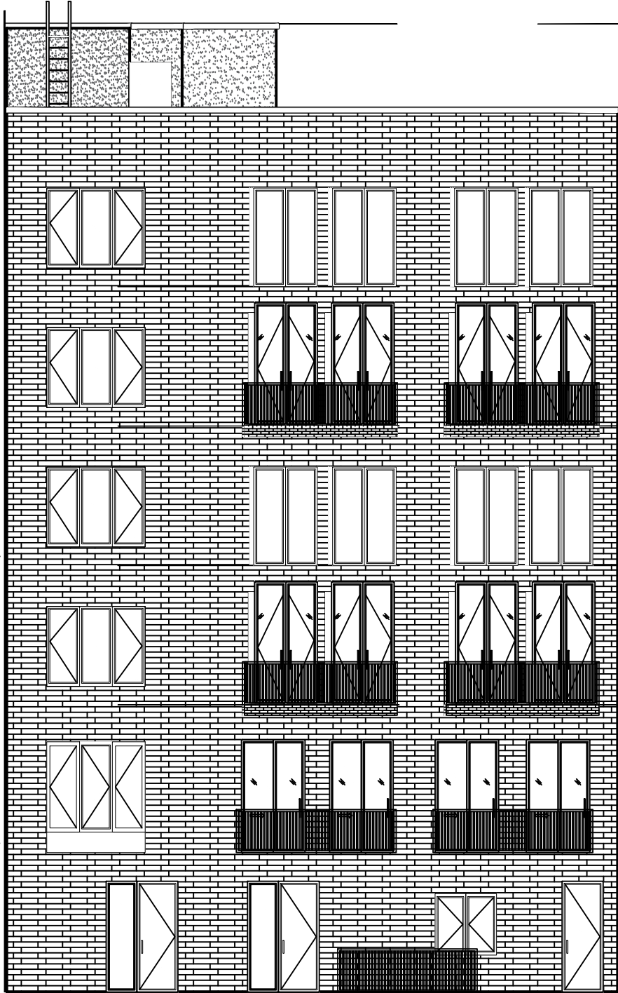
66 GERRY STREET FRONT ELEVATION
