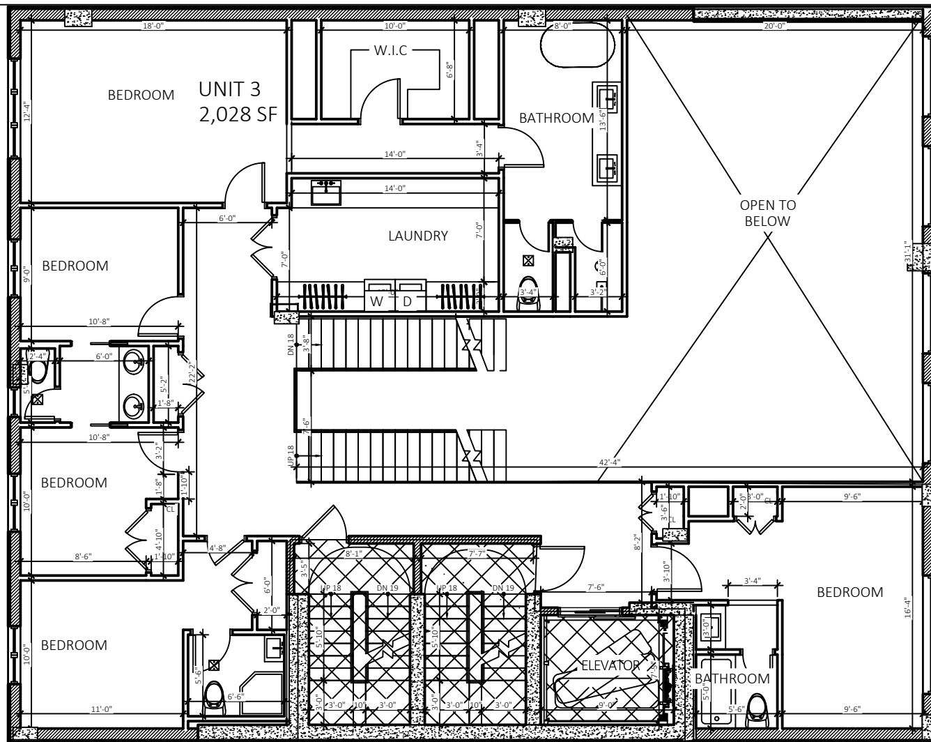
6TH FLOOR PLAN-UNIT 3
