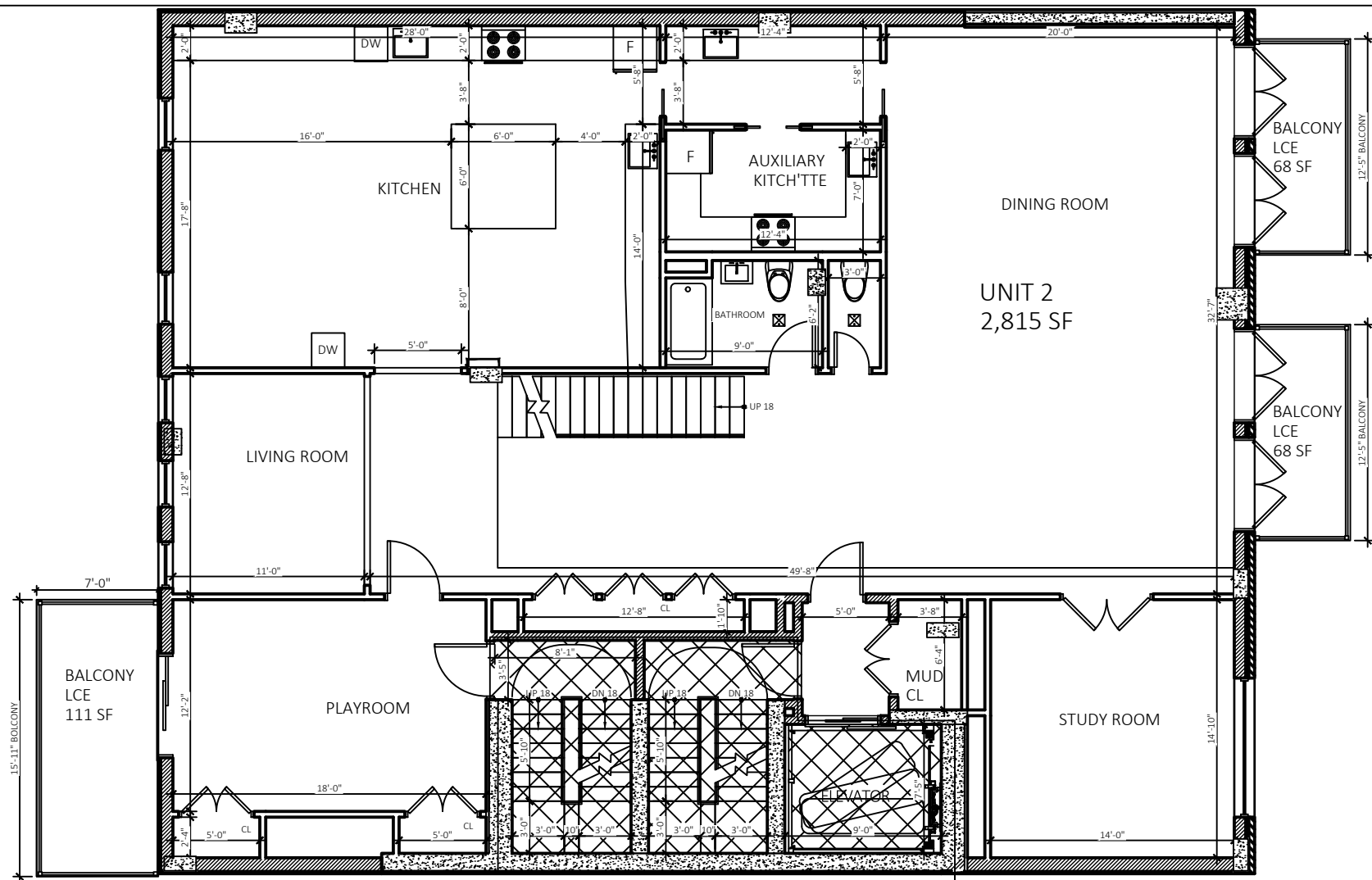
3RD FLOOR PLAN-UNIT 2
