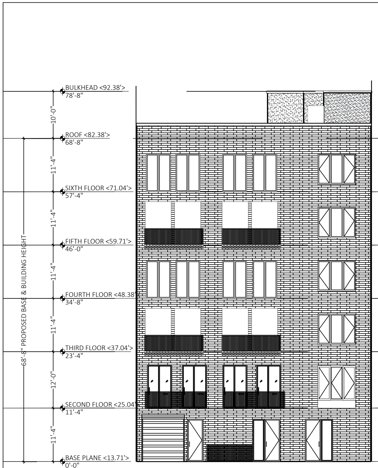
60 GERRY STREET FRONT ELEVATION
