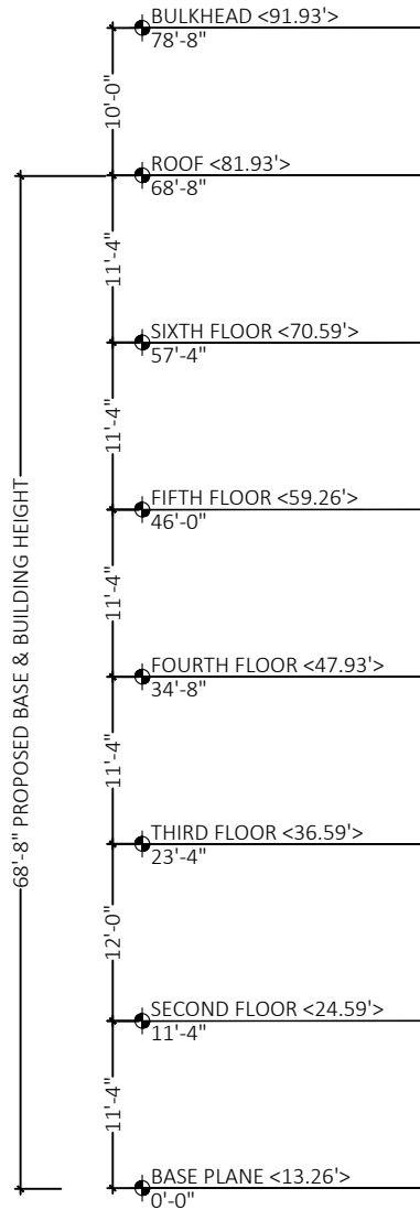
60 GERRY STREET SIDE ELEVATION
