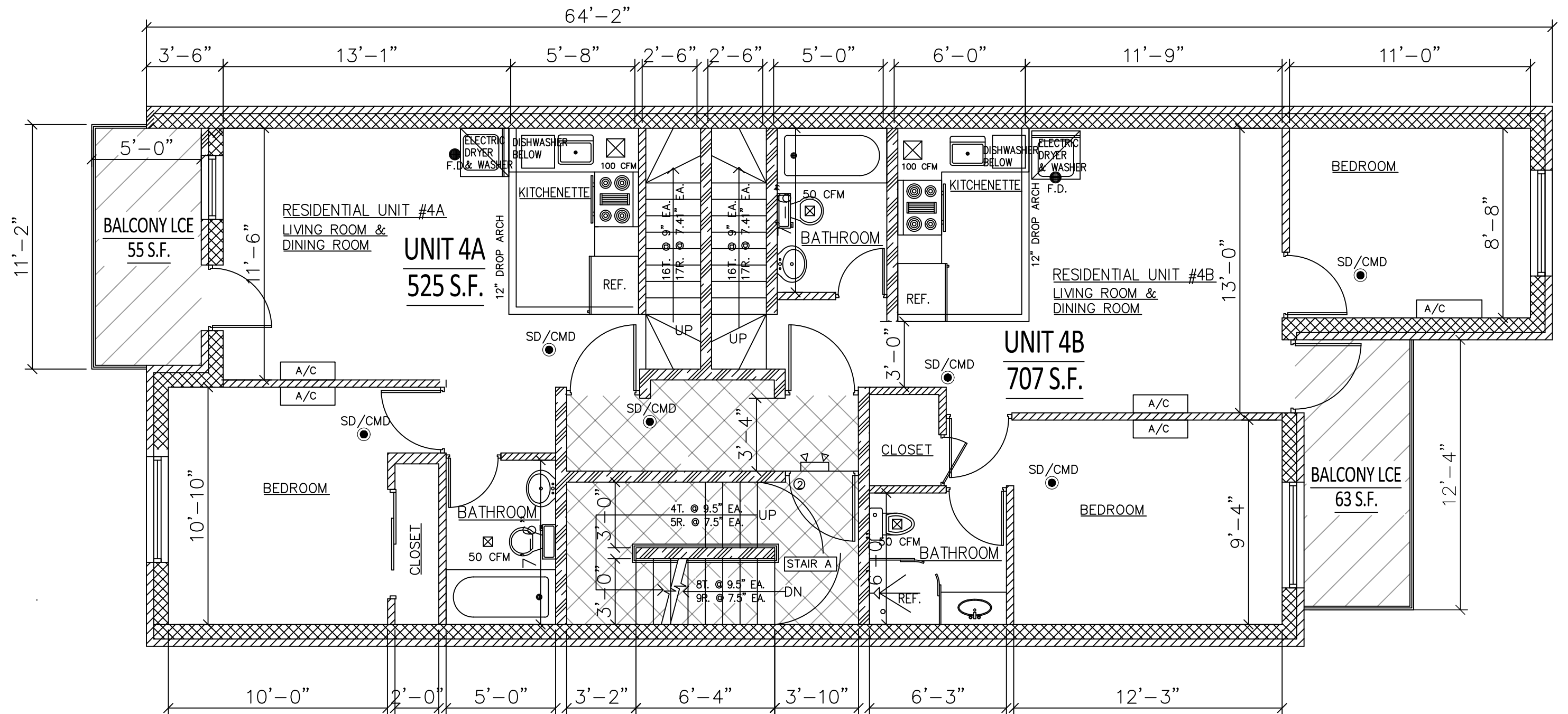
4TH FLOOR PLAN
