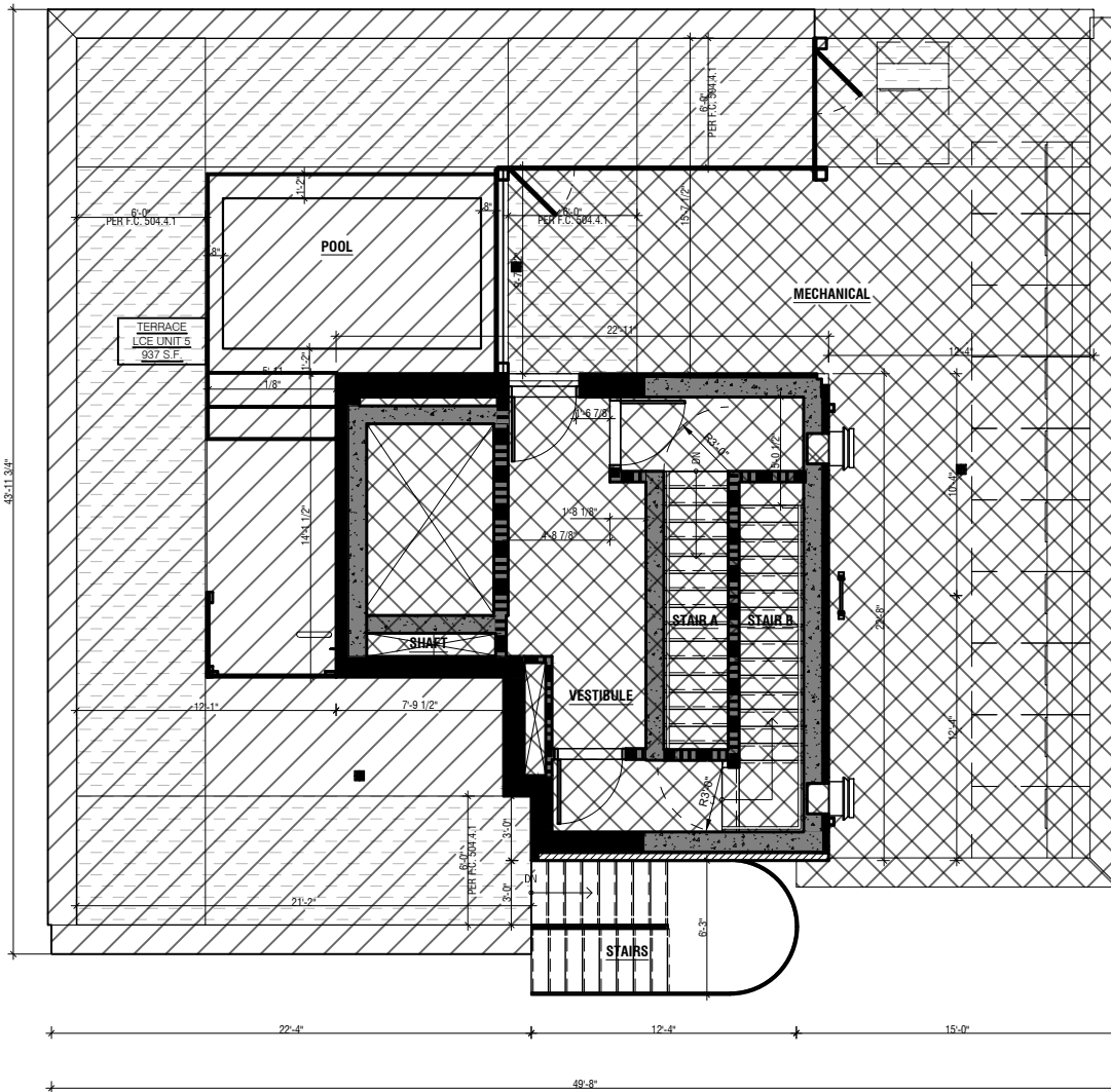
ROOF FLOOR PLAN
