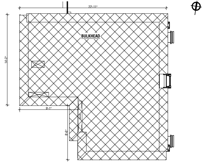
BULKHEAD FLOOR PLAN
