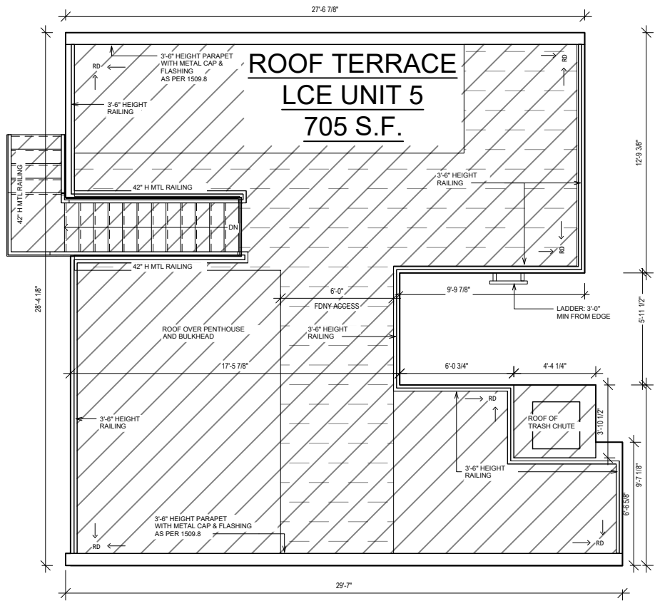
ROOF FLOOR PLAN
