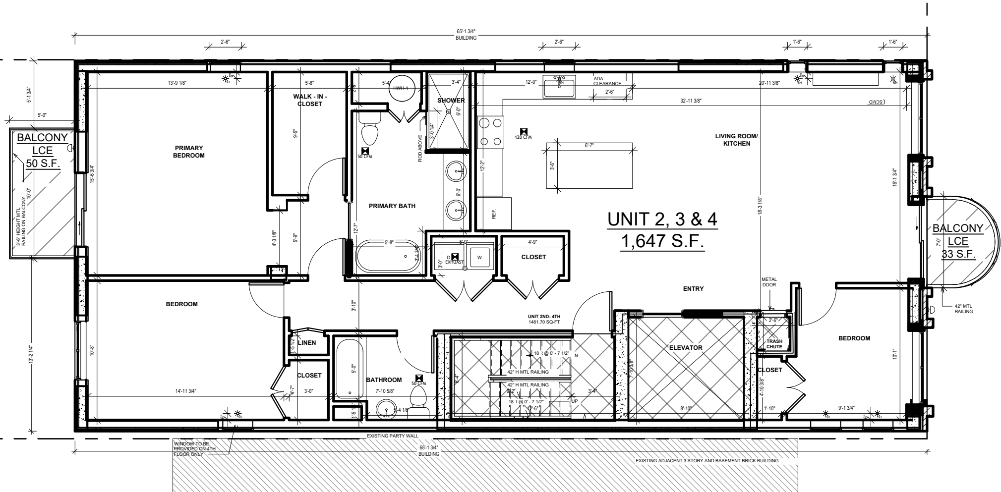
SECOND THROUGH FOURTH FLOOR PLANS
