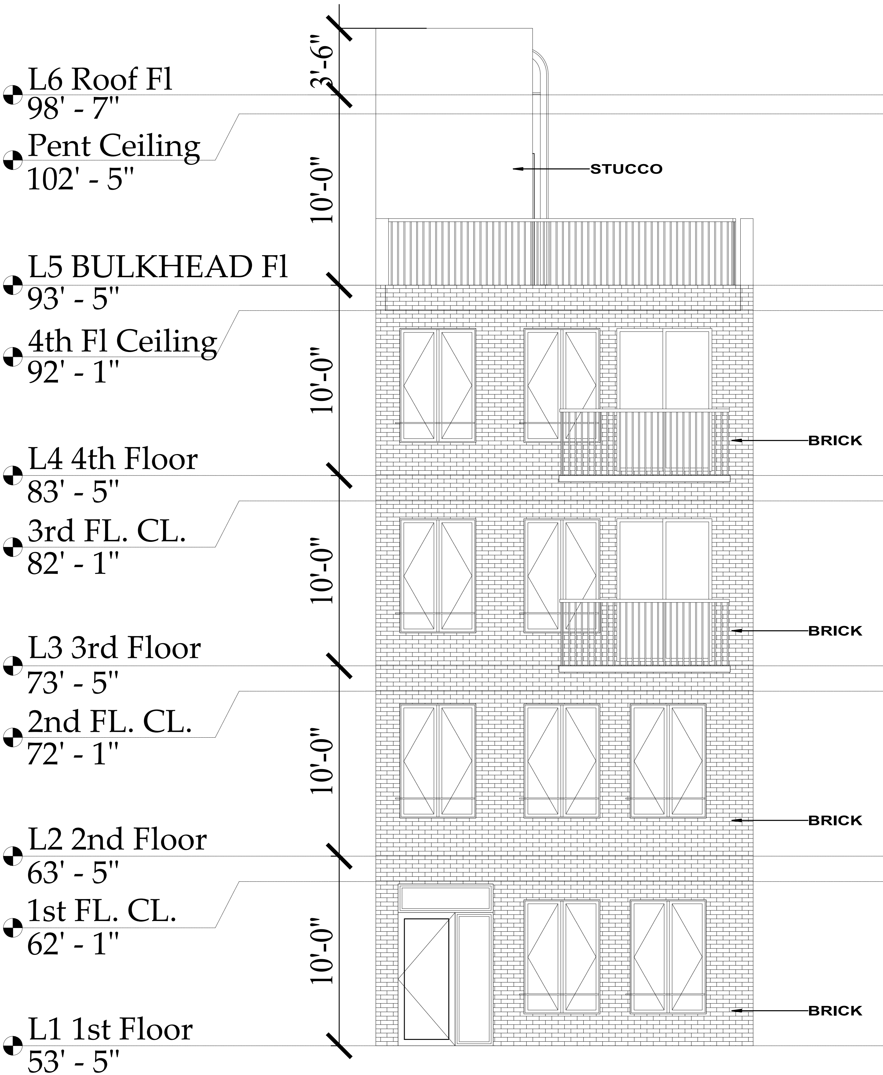
FRONT ELEVATION (SOUTH)
