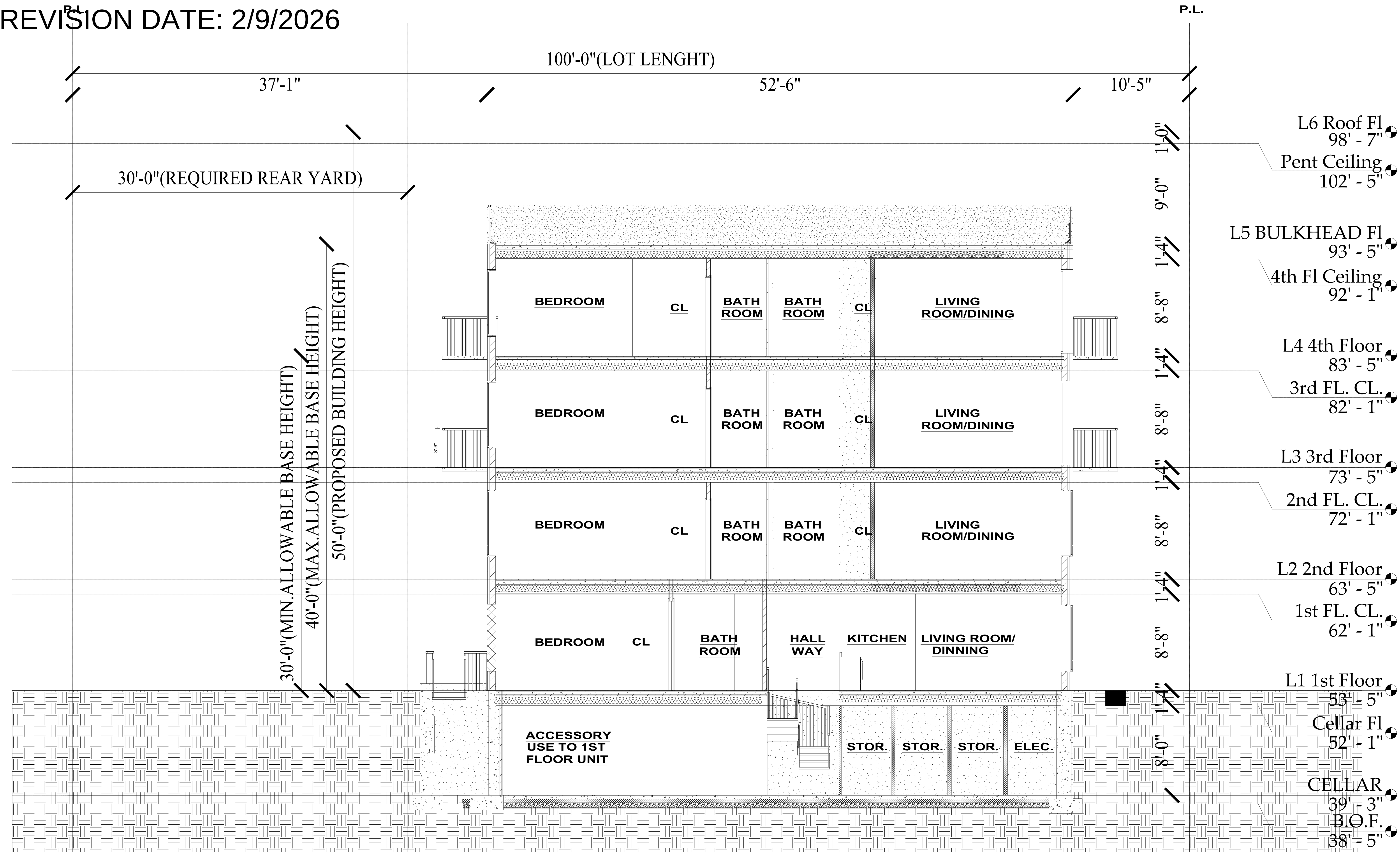
SECTION PLAN
