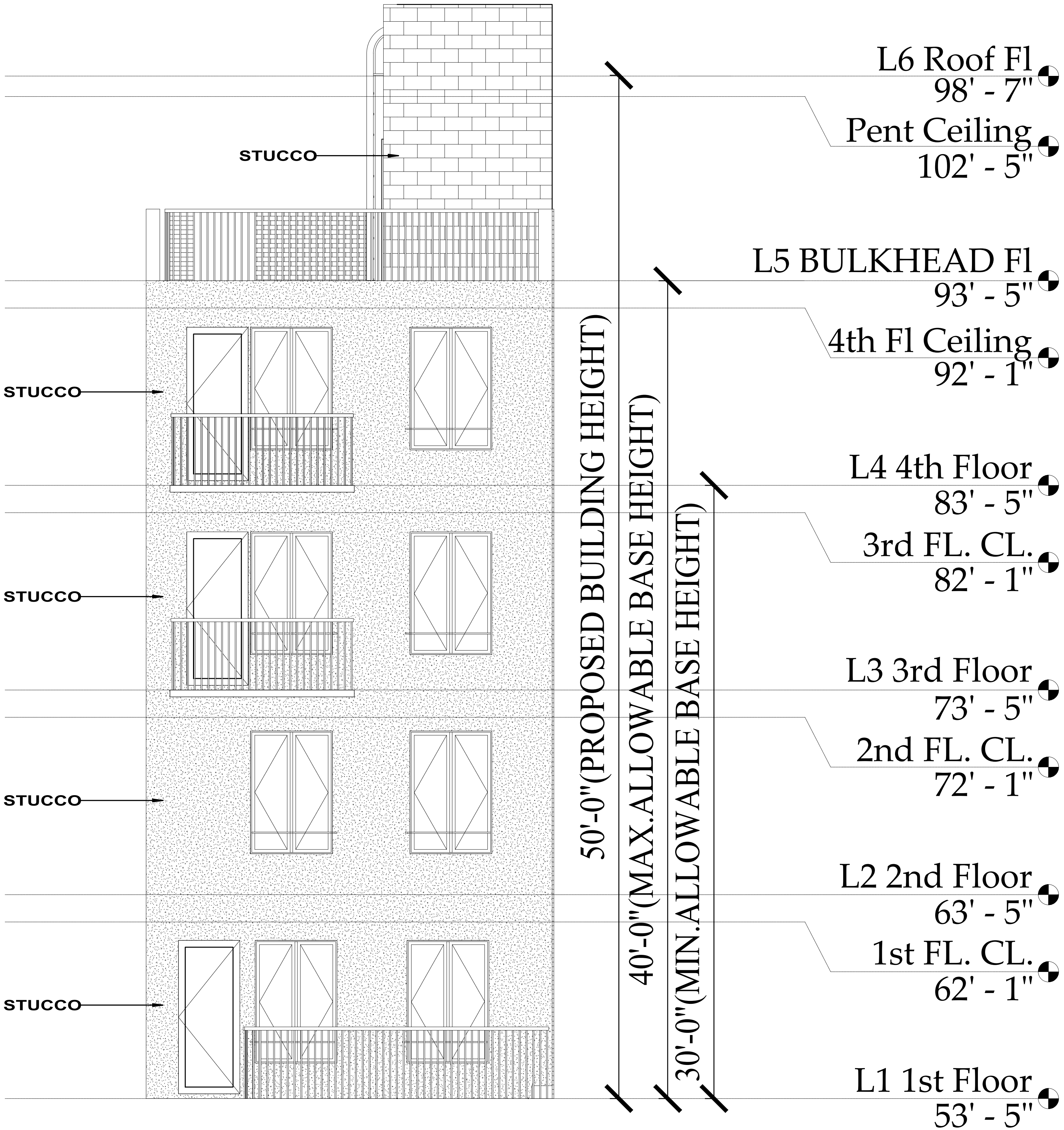
BACK ELEVATION (NORTH)
